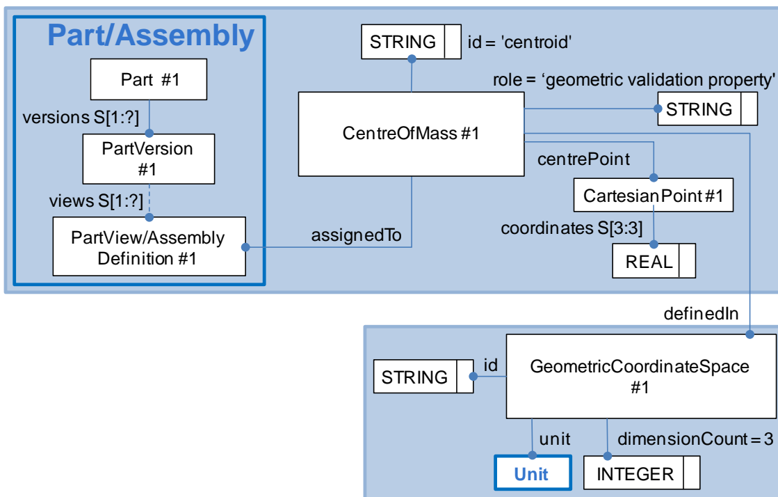
Figure 55: GVP 'centroid' or CentreOfMass assigned to a Part or Assembly
