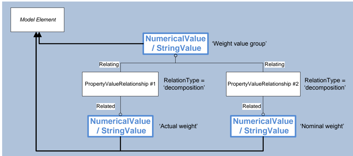
Figure 45: Defining a group of attribute values
