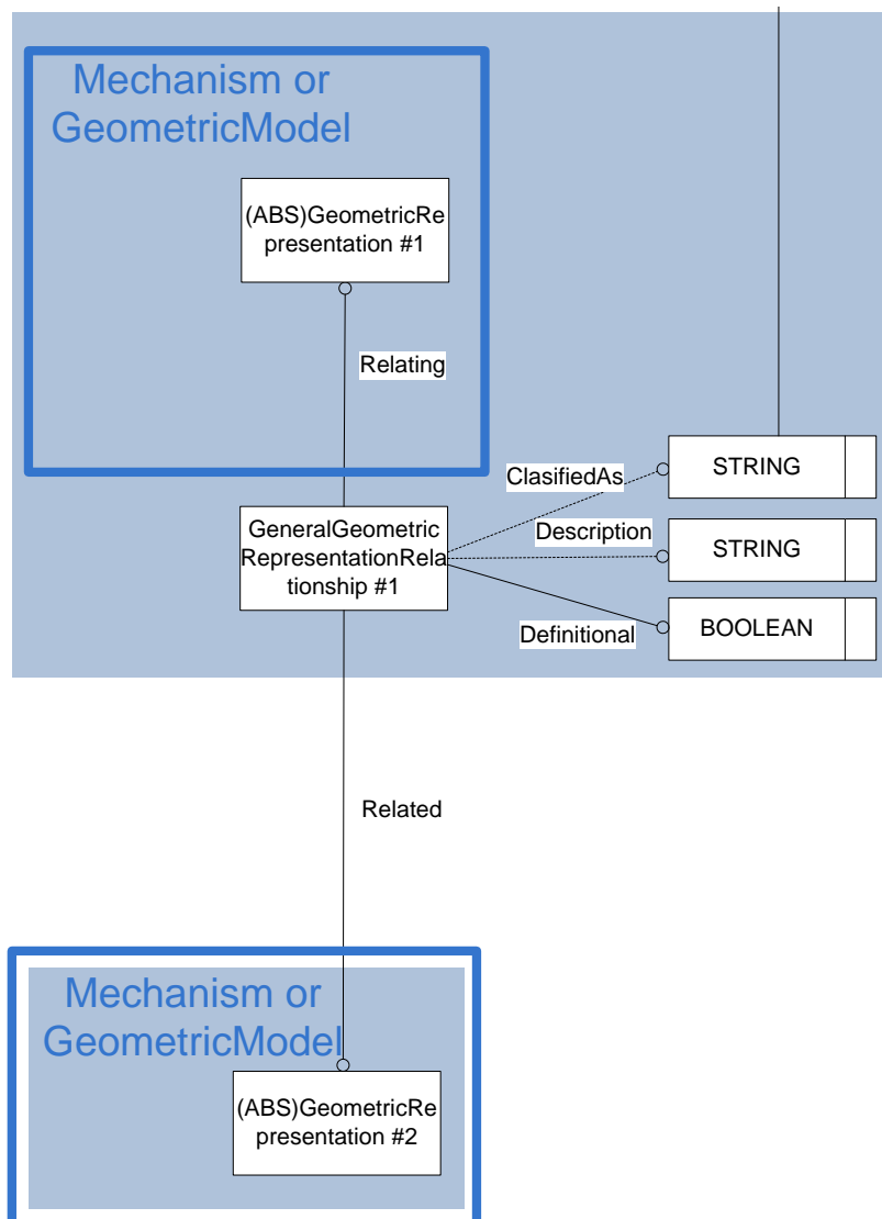
Figure 26: General Geometric Representation Relationship
