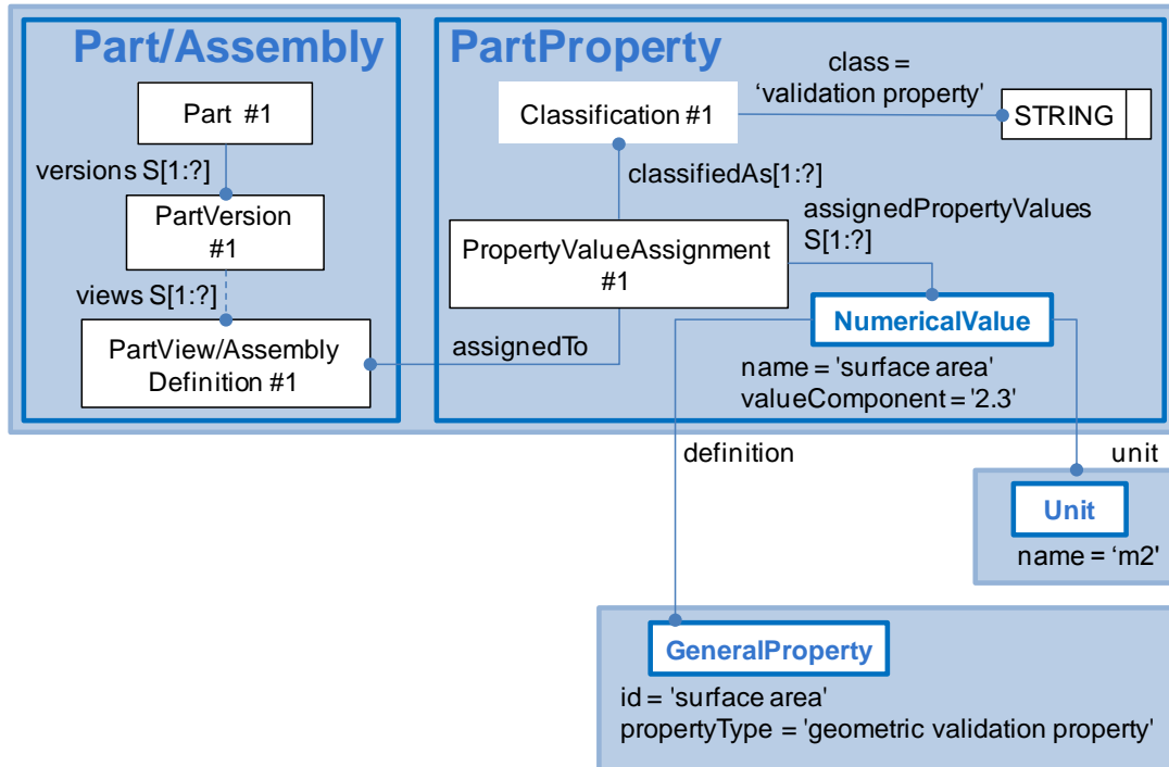
Figure 54: GVP 'surface area' of 2.3 squaremetre assigned to a Part or Assembly
