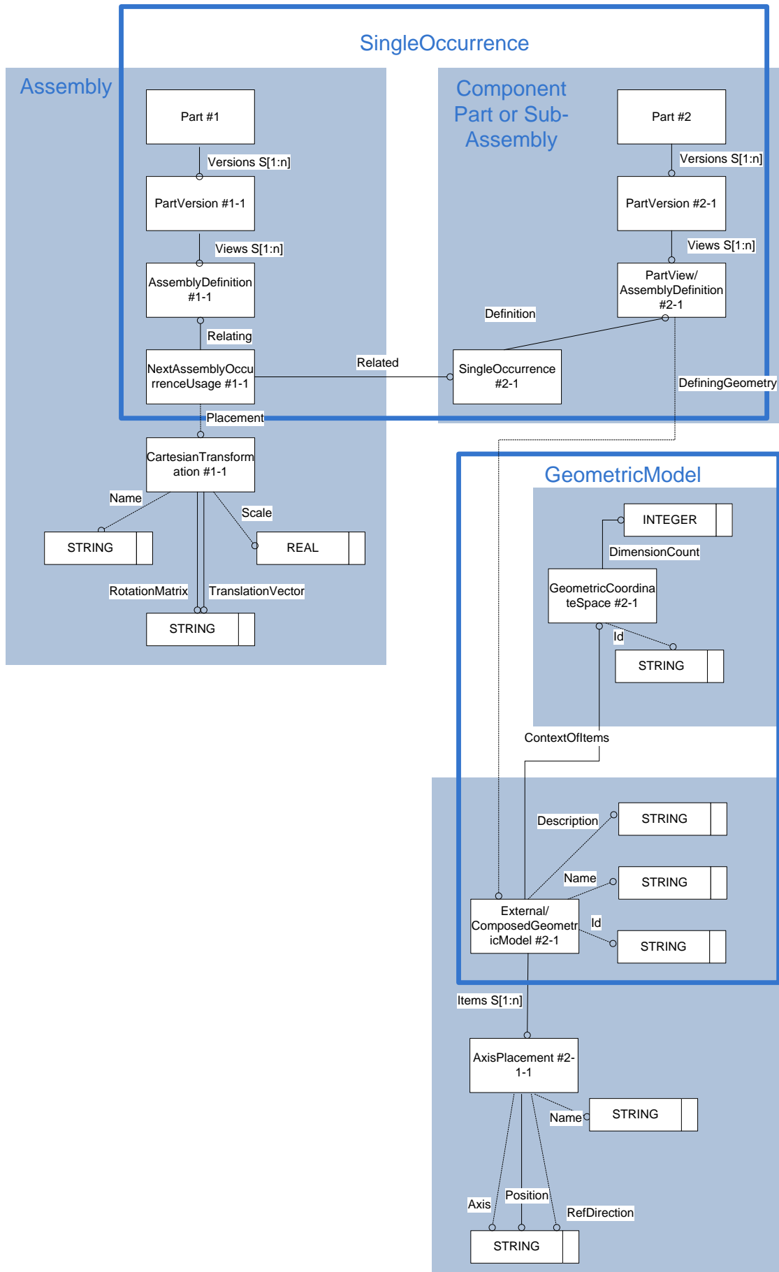
Figure 21: Template "Simplified Positioning Representation"
