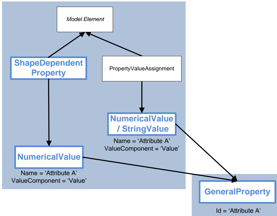
Figure 42: Definition of an attribute name and its usage
