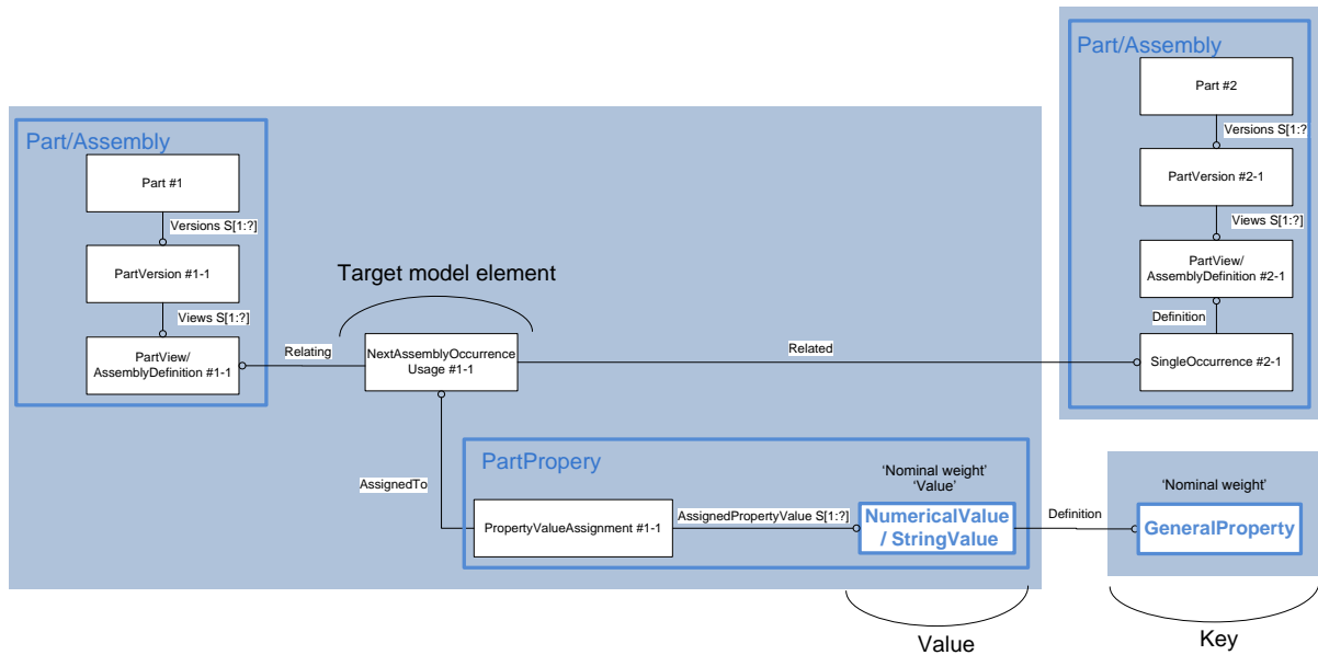
Figure 47: User defined attribute for a simple component instance in an assembly
