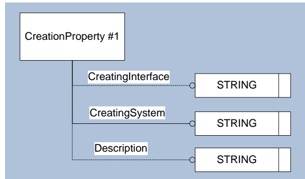
Figure 37: Template “CreationProperty”
