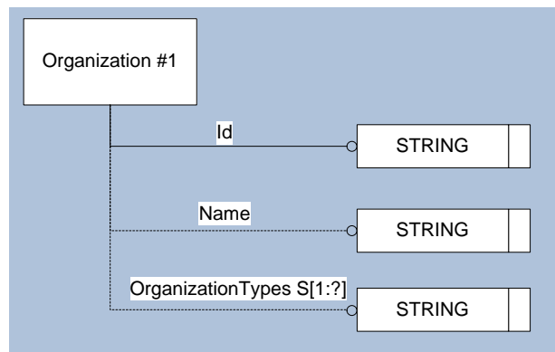
Figure 2: Template "Organization"
