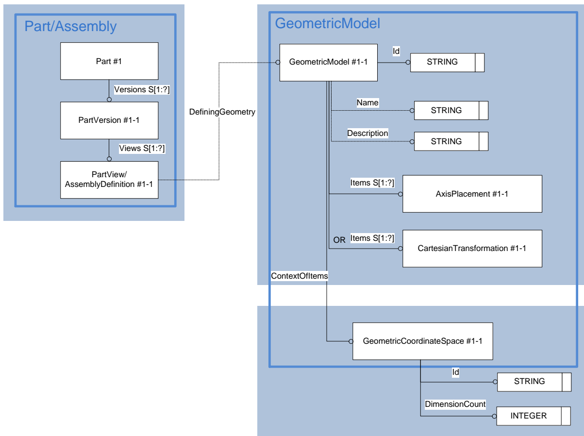
Figure 17: Template "GeometricModel"
