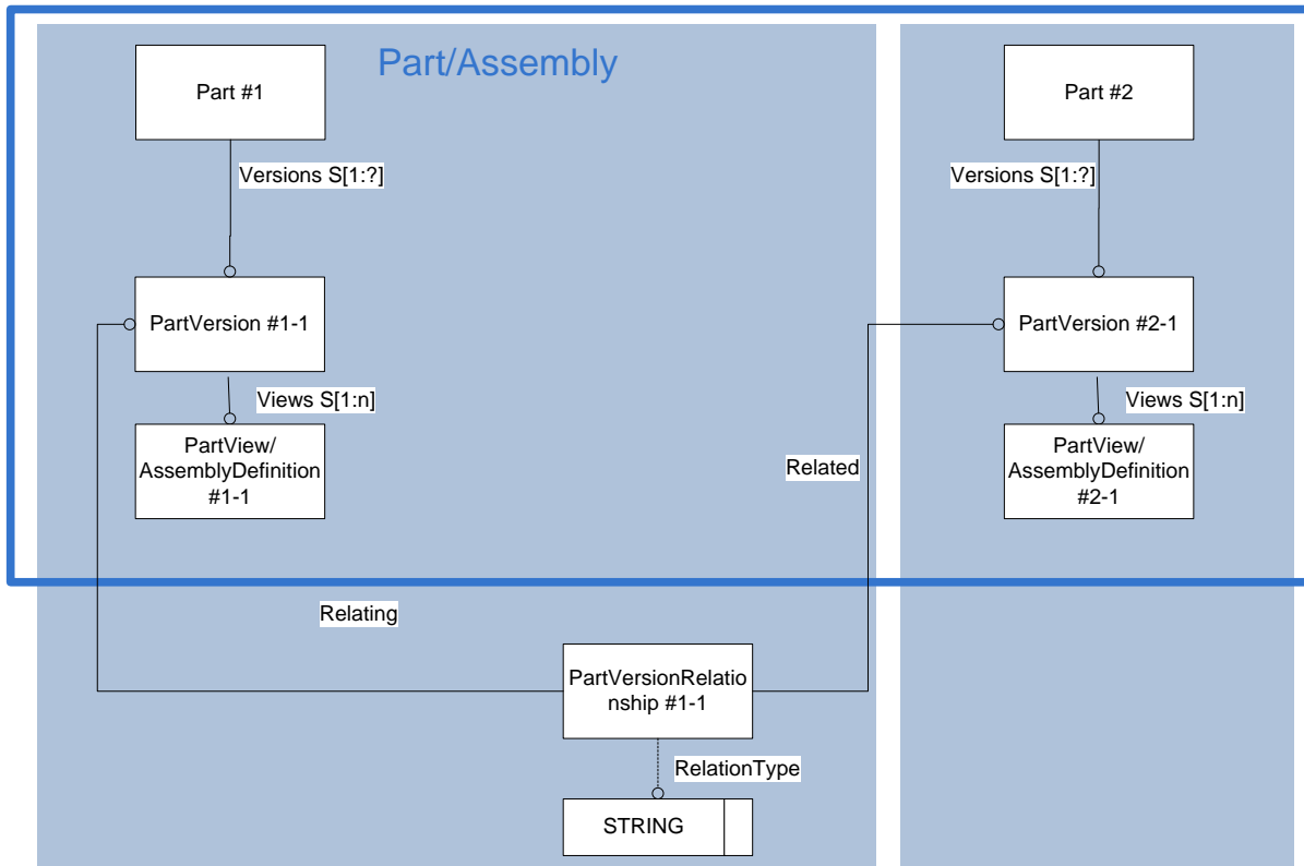
Figure 16: Template "PartVersionRelationship"
