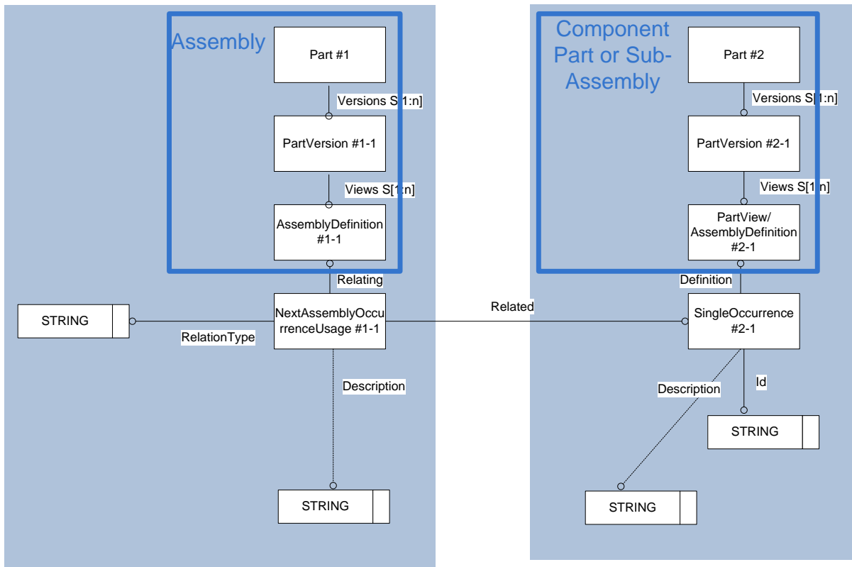
Figure 20: Template "SingleOccurrence"
