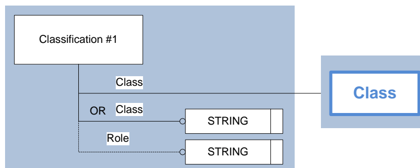
Figure 5: Template "Classification"
