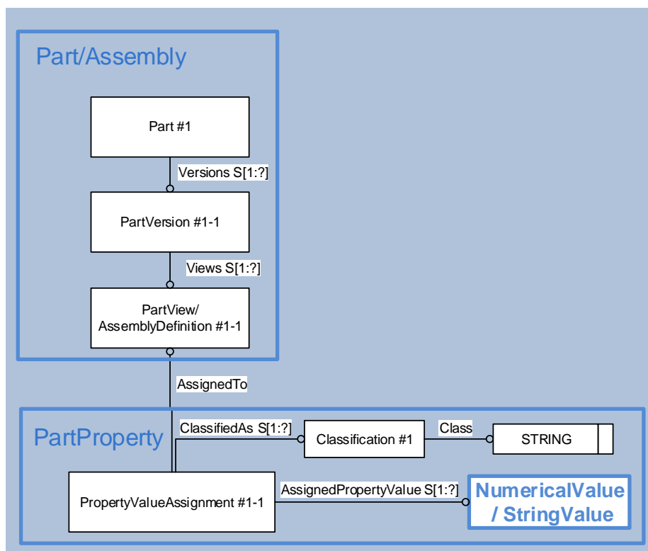
Figure 18: Template "PartProperty"
