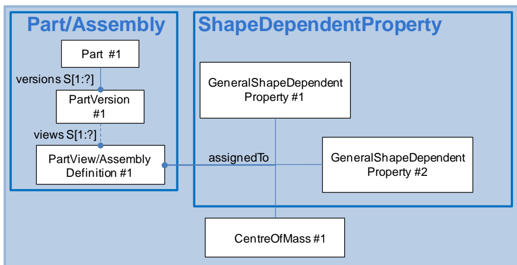
Figure 52: Geometric Validation Properties at the Part and Assembly level
