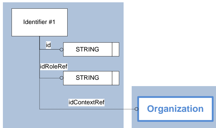
Figure 6: Template "Identifier"
