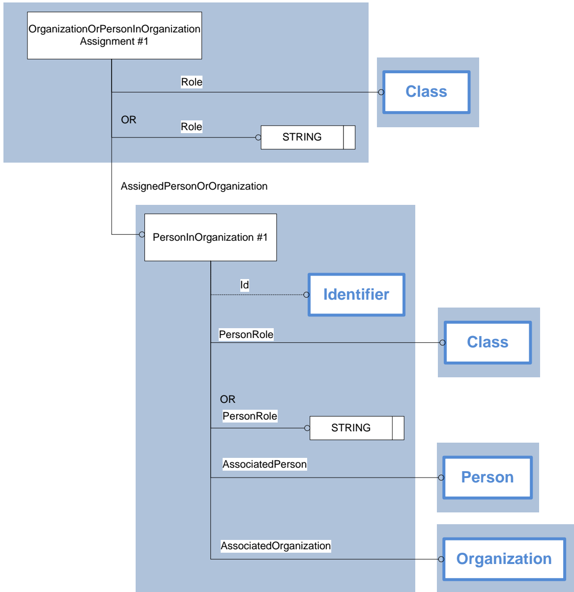
Figure 13: Template “PersonInOrganization”
