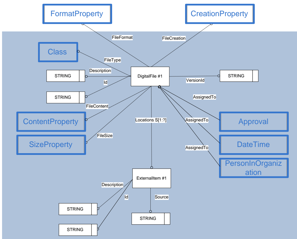
Figure 29: Template "DigitalFile"
