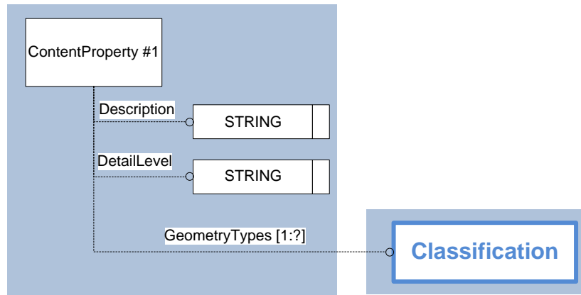
Figure 36: Template “ContentProperty”
