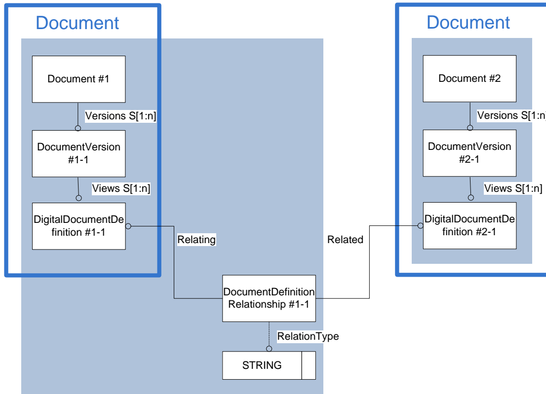
Figure 28: Template "DocumentDefinitionRelationship"
