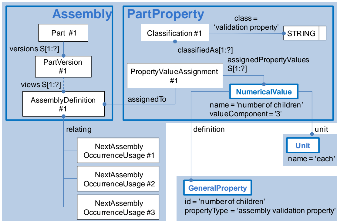
Figure 50: Instantiation of AVP ‘number of children’ for 3 children
