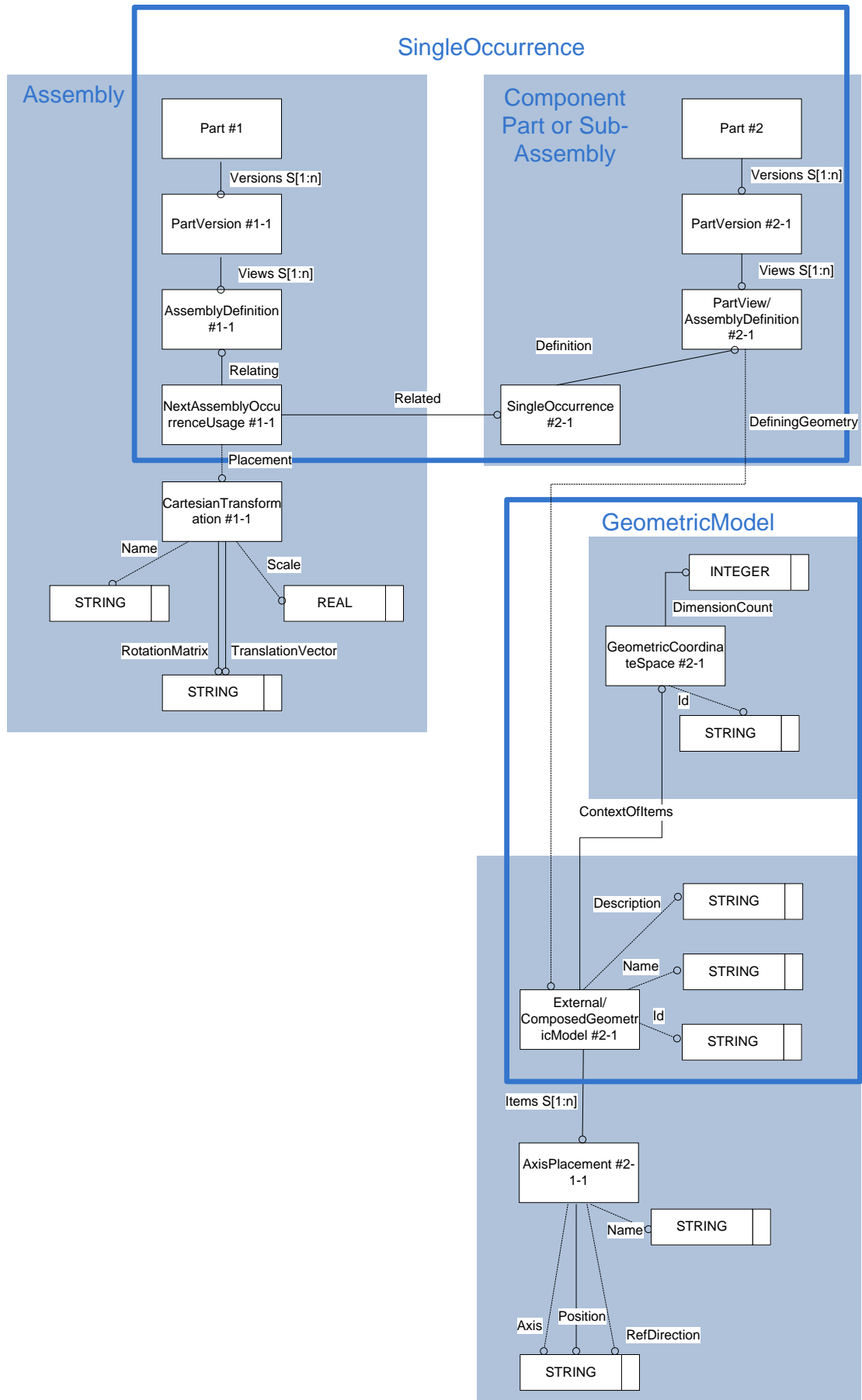
Figure 22: Instantiation example if Part #2 has geometry
