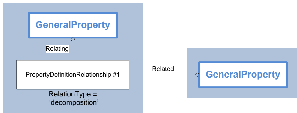
Figure 44: Defining a group of attributes
