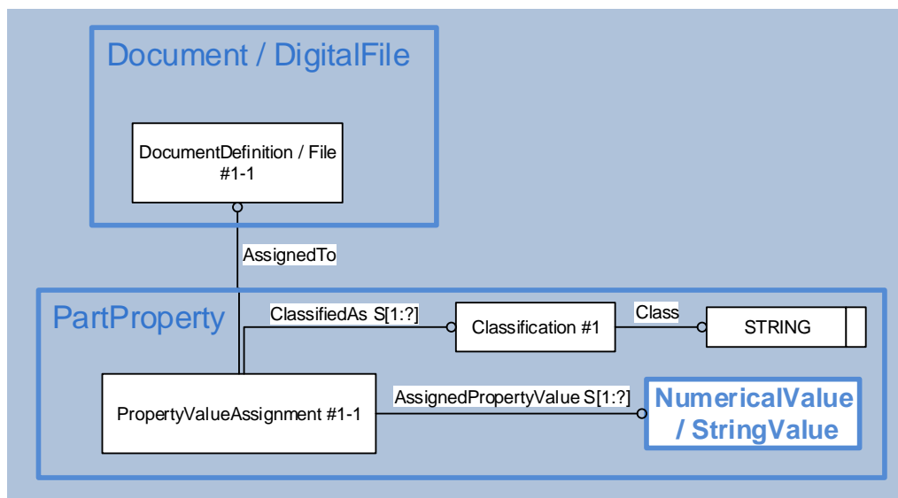
Figure 39: Template "DocumentFileProperty"
