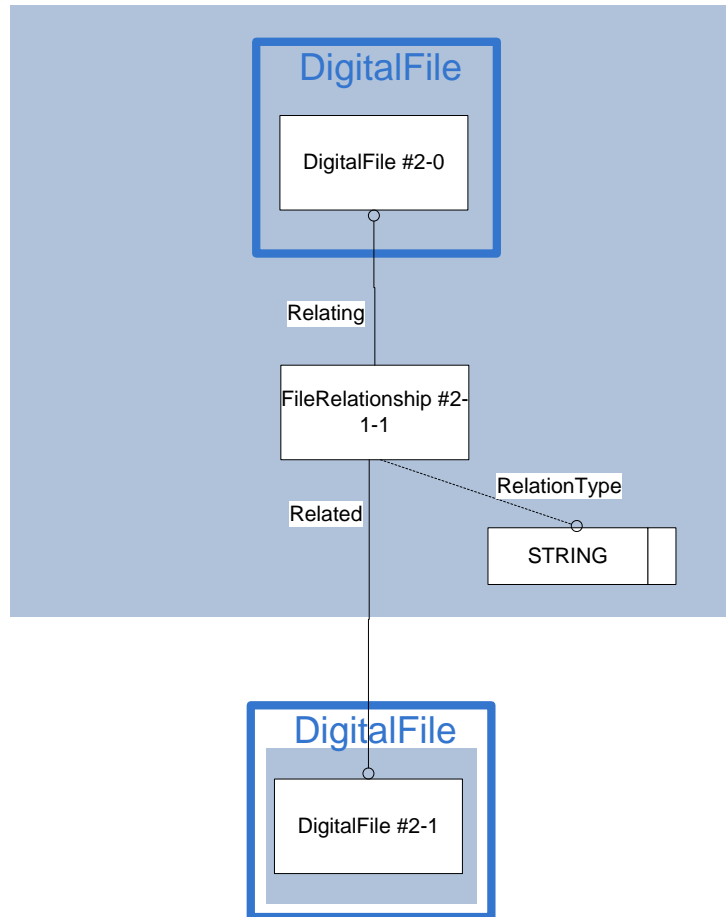
Figure 30: Template “FileRelationship”
