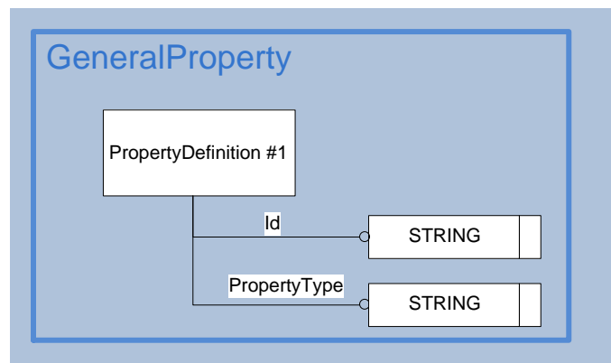
Figure 43: Template "GeneralProperty"
