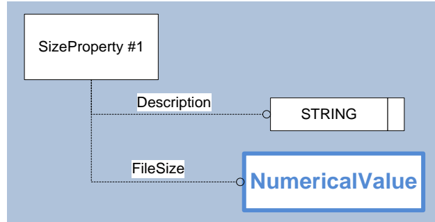
Figure 38: Template “SizeProperty”
