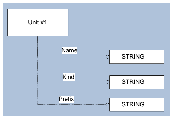
Figure 3: Template "Unit"
