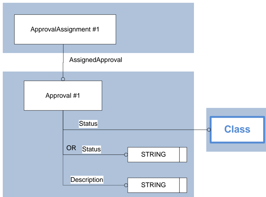
Figure 11: Template “Approval”
