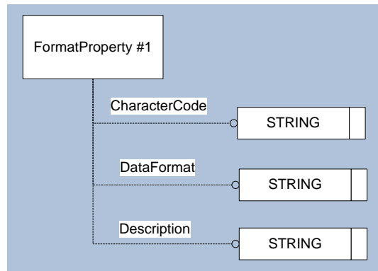
Figure 35: Template “FormatProperty”
