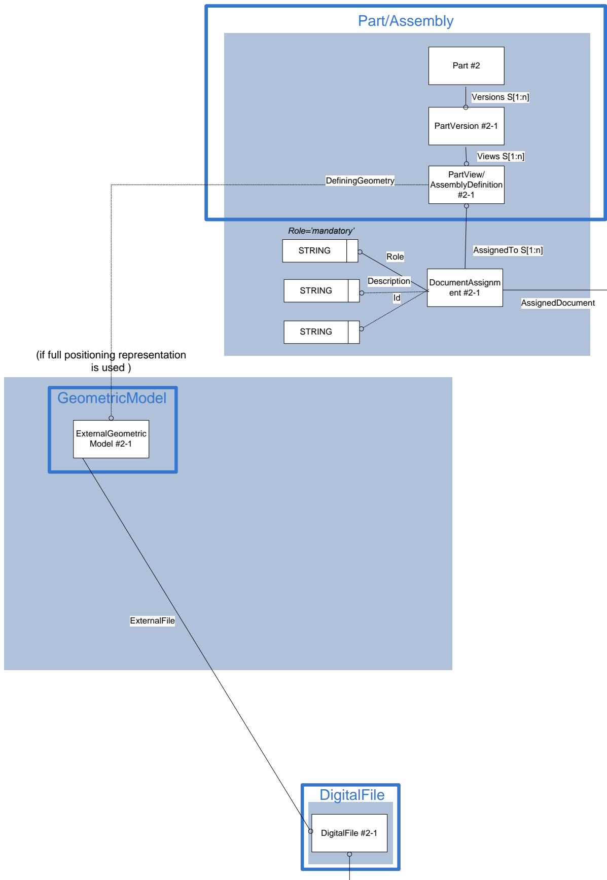
Figure 40: Template "CAx Representation for DocumentAssignment"
