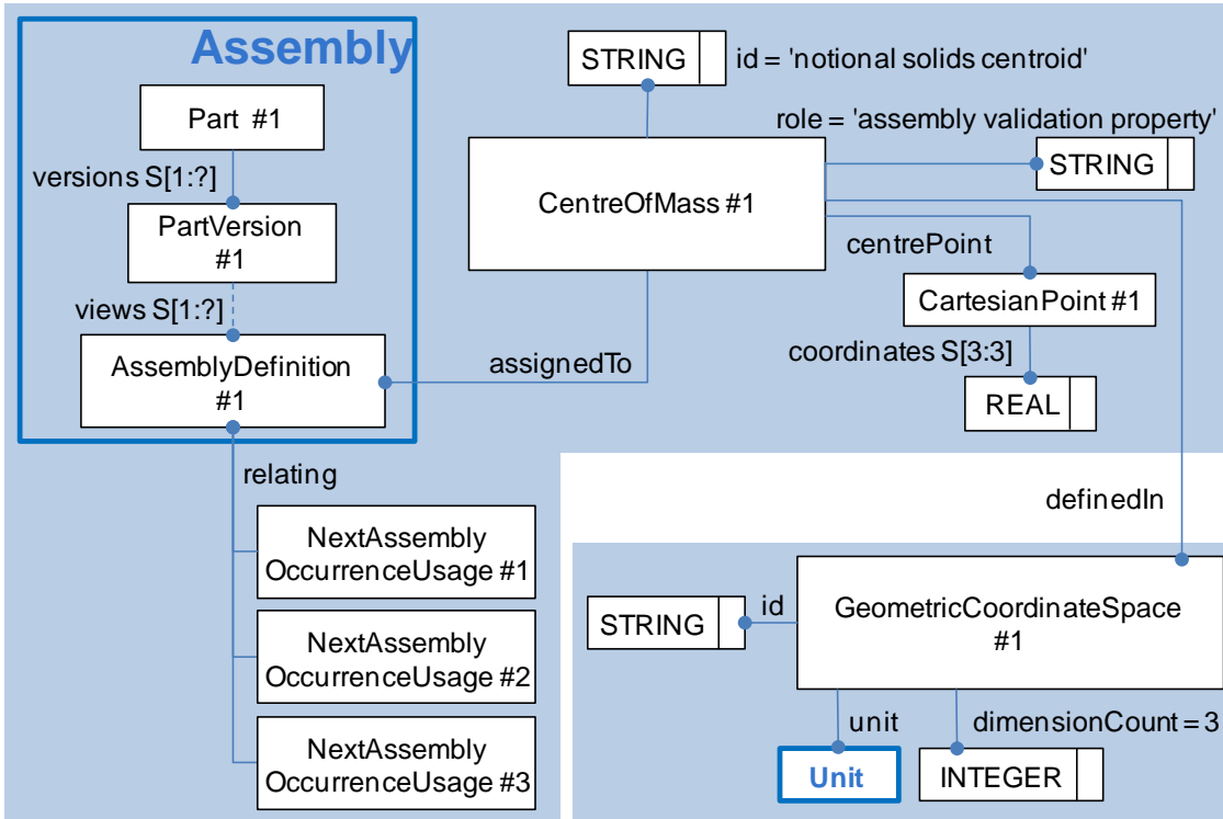
Figure 51: Instantiation of AVP ‘notional solids centroid’
