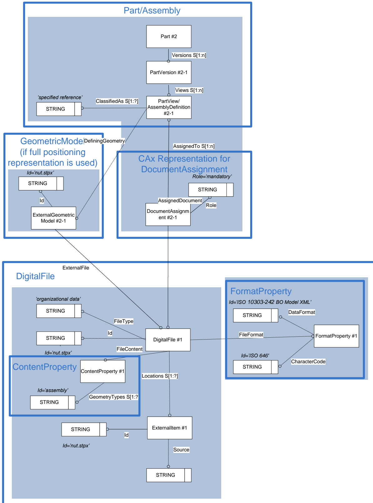
Figure 33: Element Structure for Nested XML File (using CAX representation)
