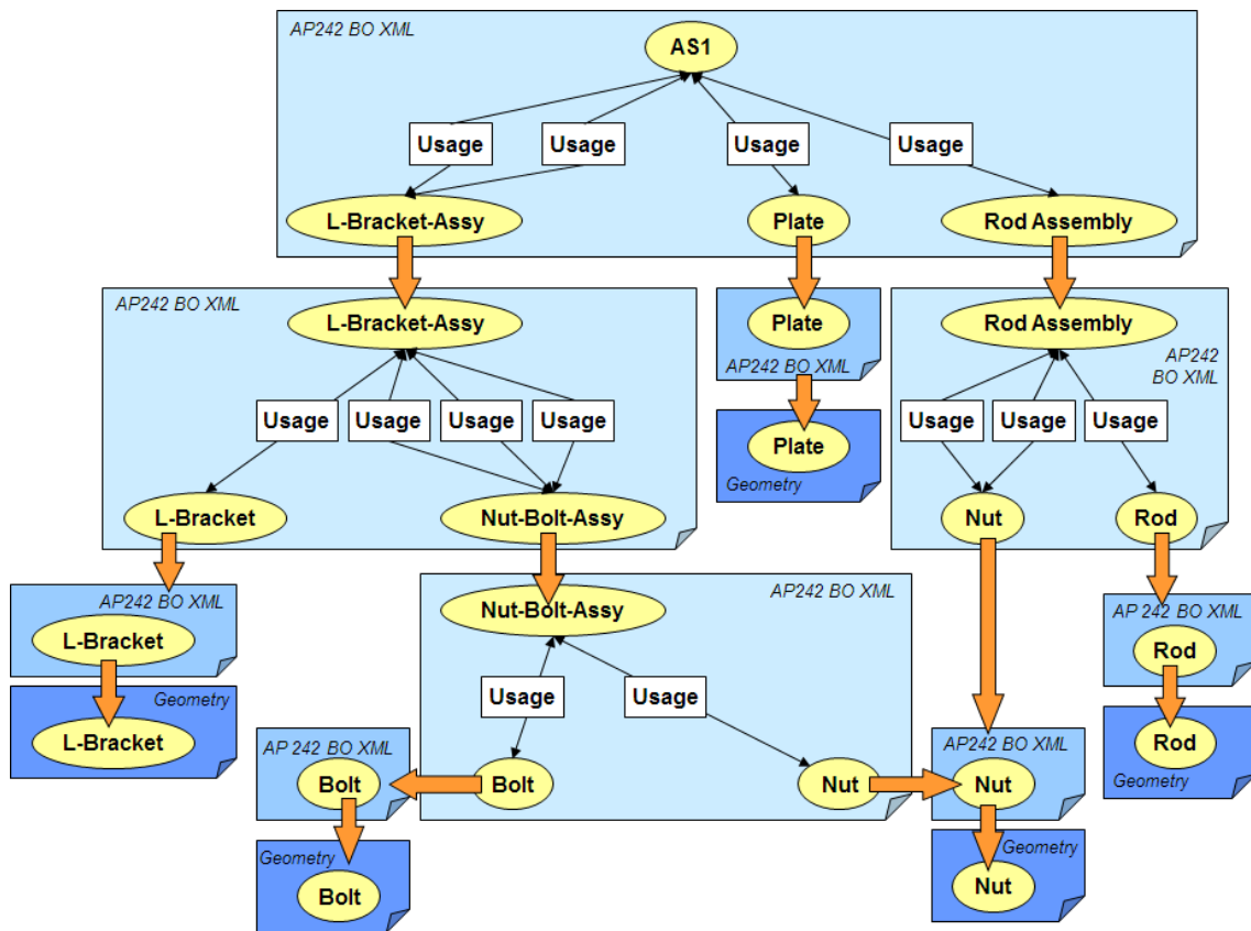
Figure 32: Example for Nested Structure with additional part-level XML files
