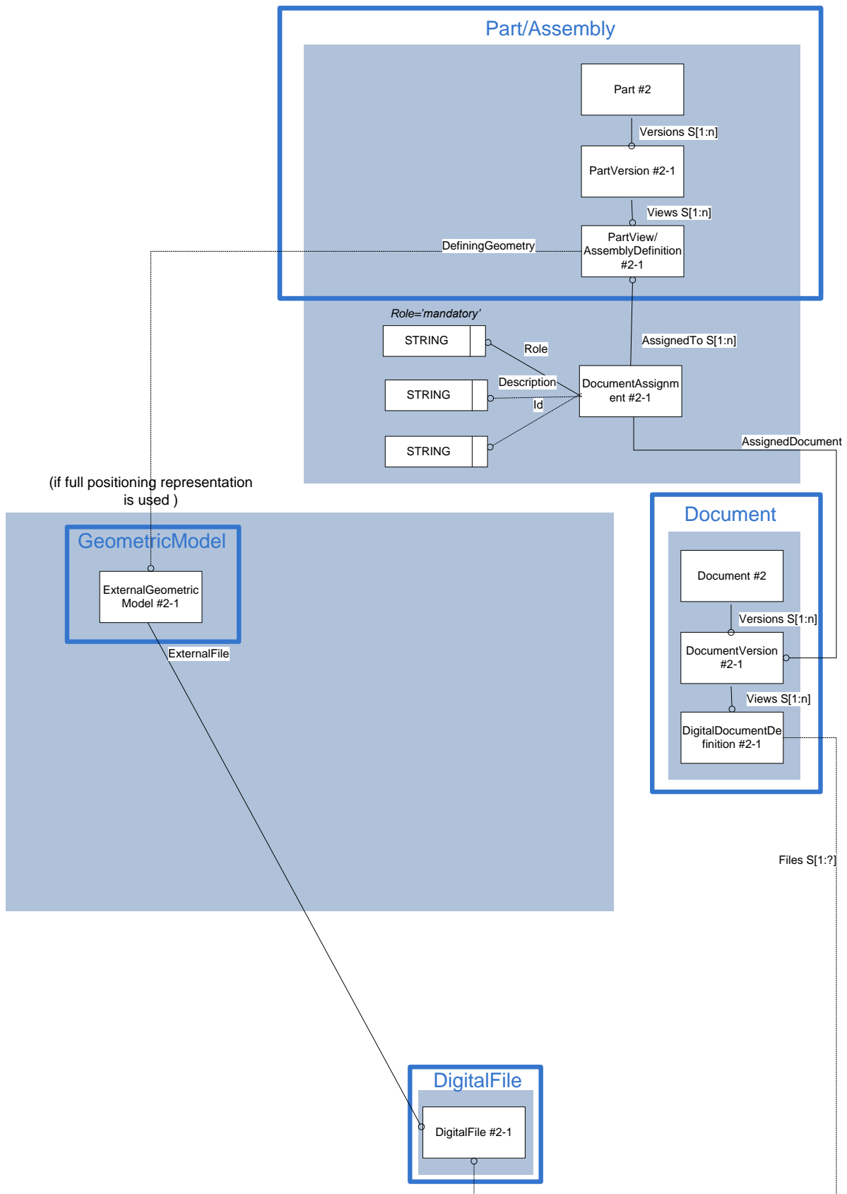
Figure 41: Template "PDM Representation for DocumentAssignment"
