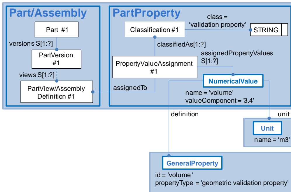
Figure 53: GVP 'volume' of 3.4 cubicmetre assigned to a Part or Assembly
