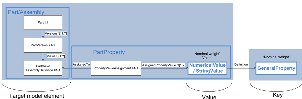
Figure 46: User defined attribute at the part/assembly level
