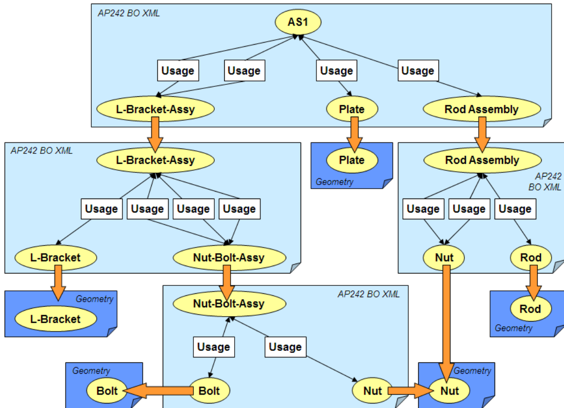
Figure 31: Example for Nested Structure
