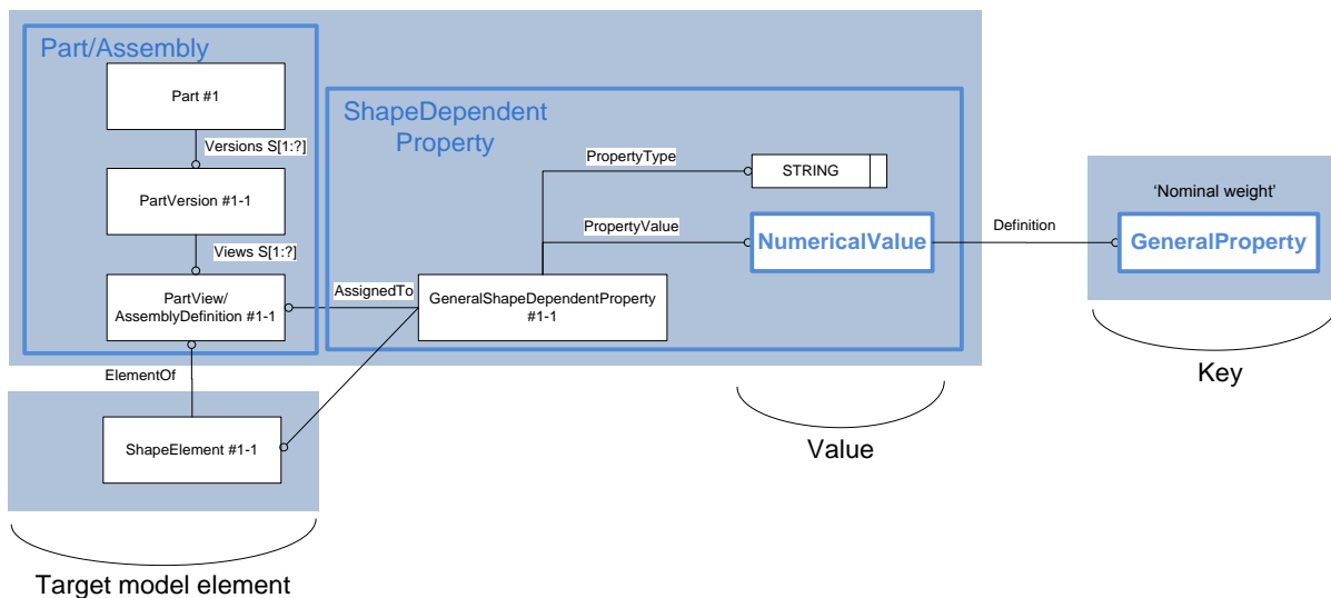
Figure 48: User defined attribute for a shape or a portion of shape
