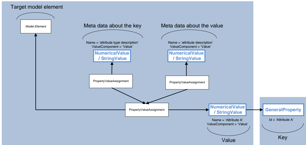
Figure 49: Specification of meta data for an attribute and its value
