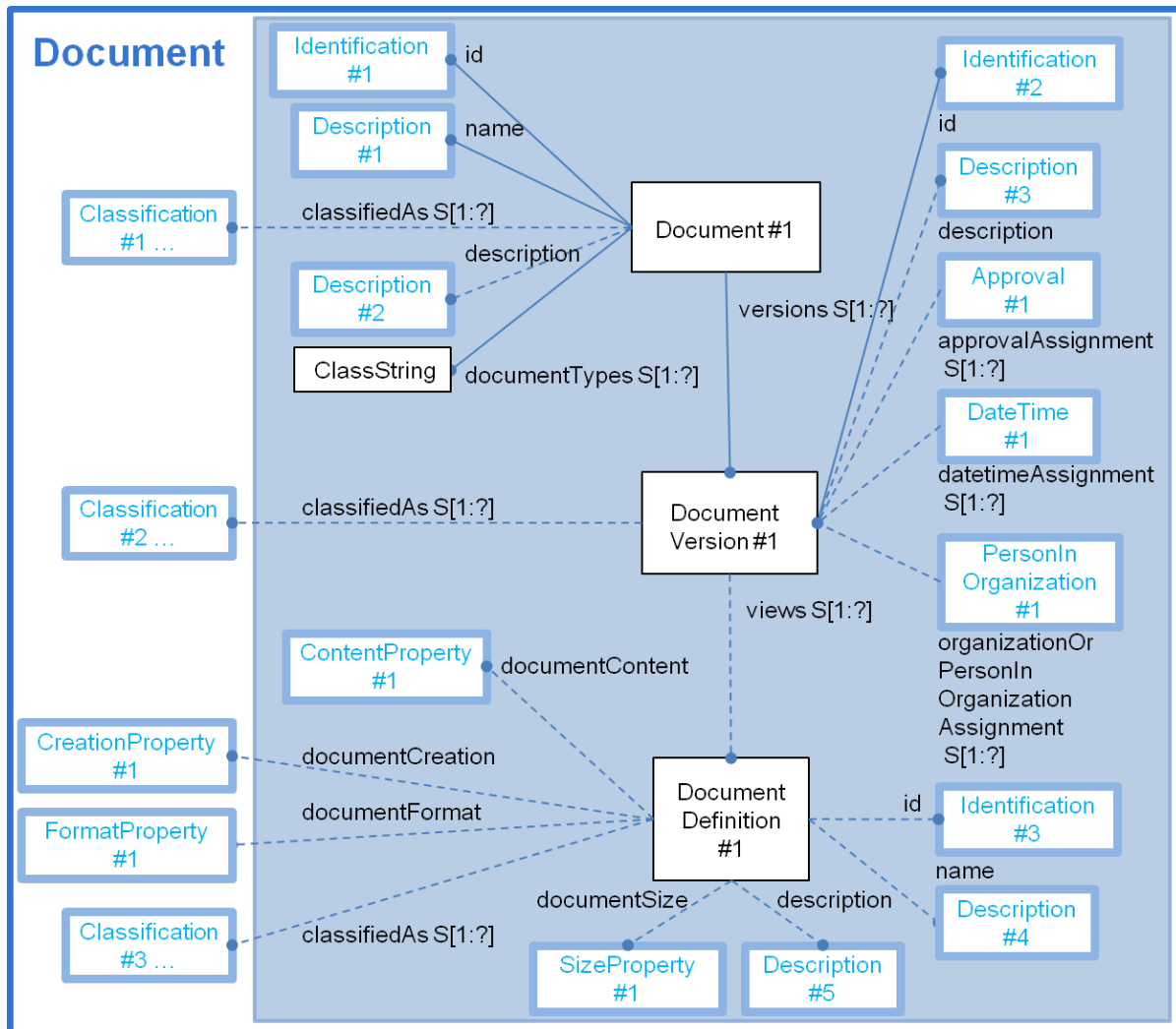
Figure 27: Template "Document"
