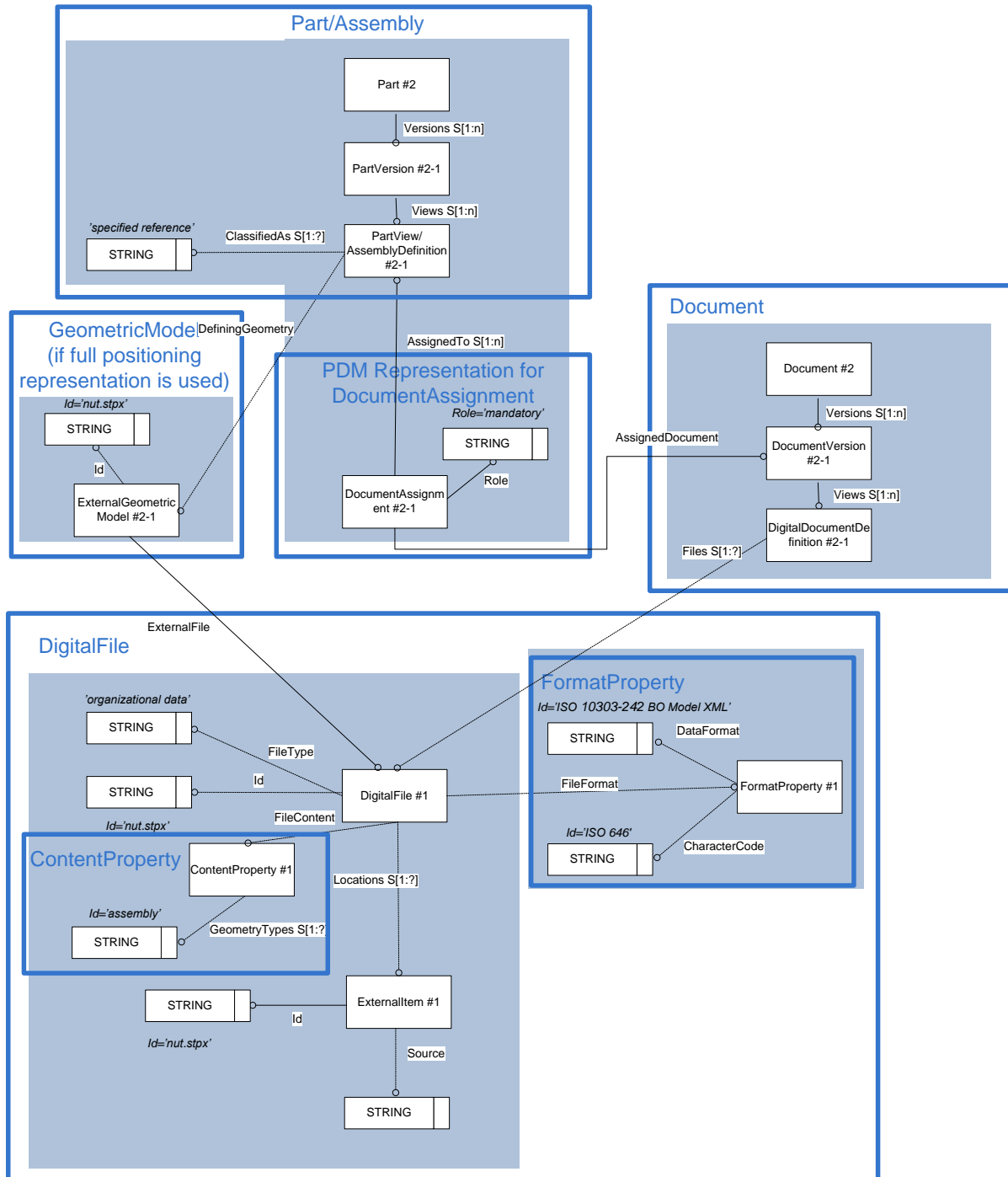
Figure 34: Element Structure for Nested XML File (using PDM representation)
