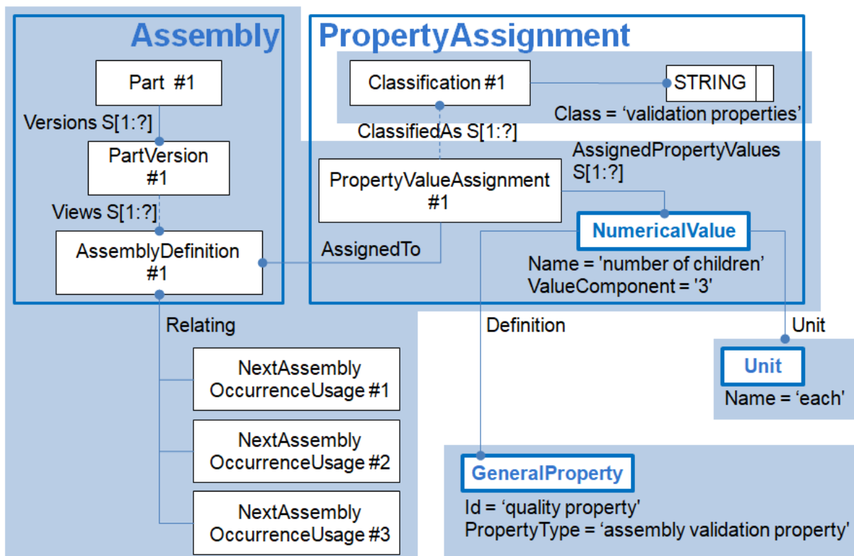
Figure 69: Instantiation of AVP ‘number of children’ for 3 children
