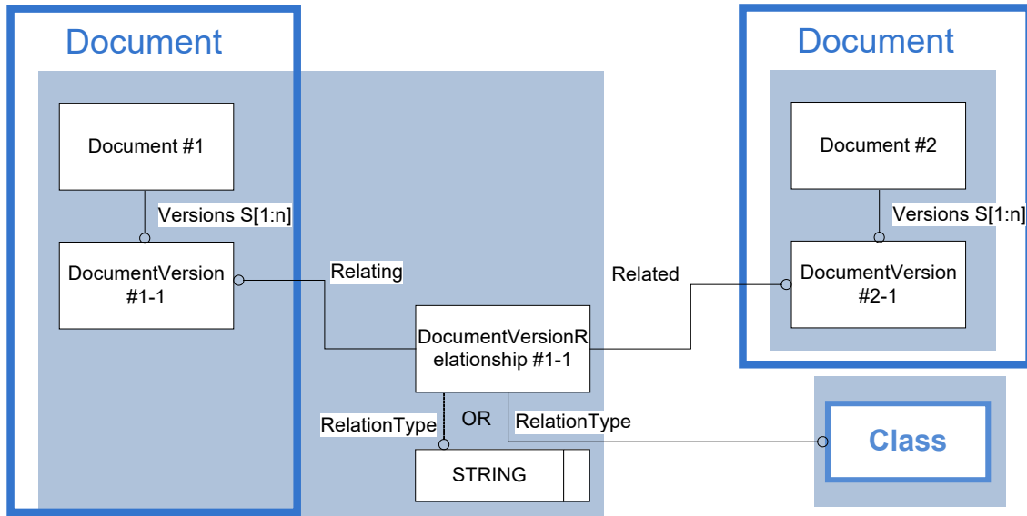
Figure 44: Template "DocumentVersionRelationship"
