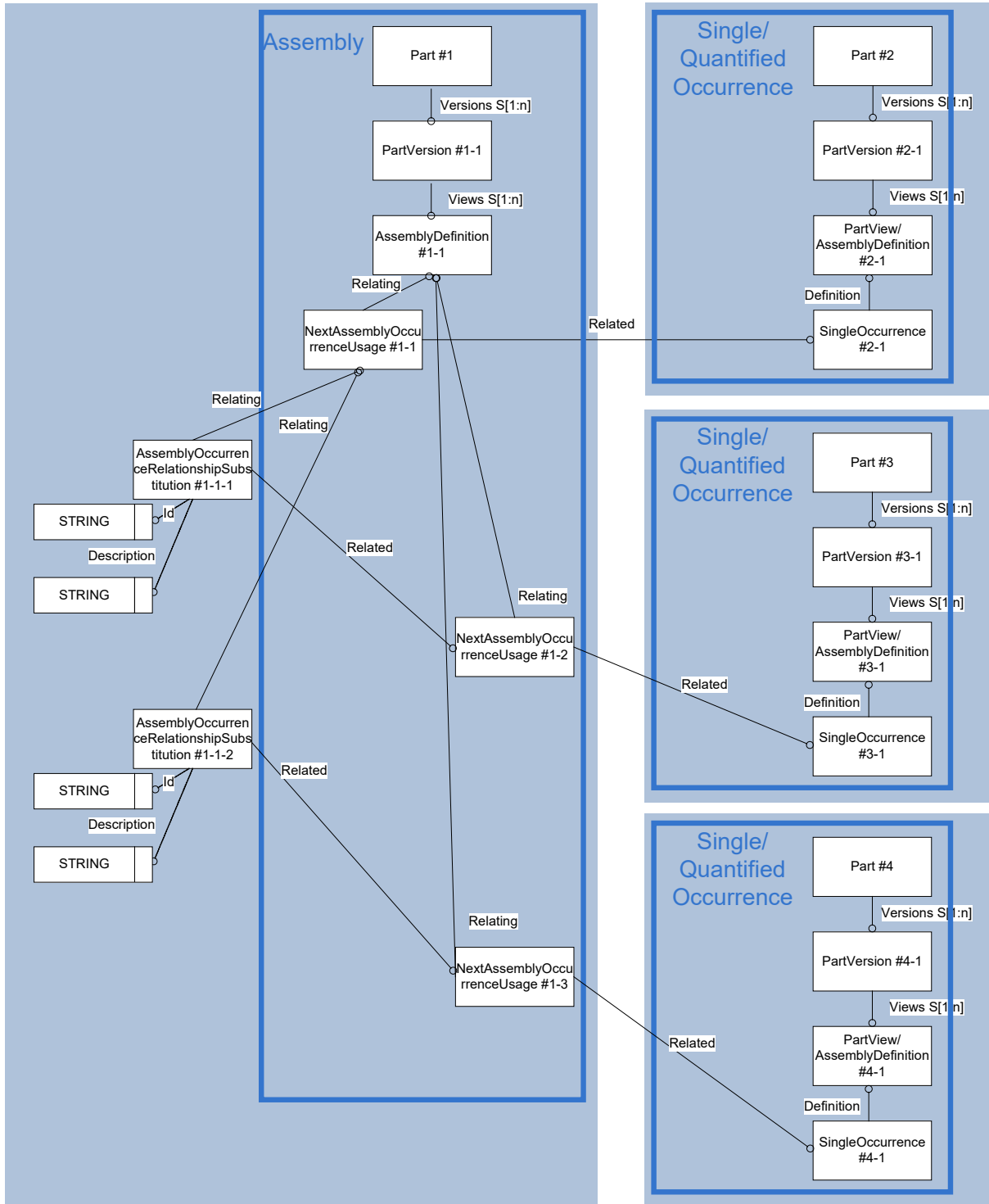
Figure 40: Template "AssemblyOccurrenceRelationshipSubstitution"
