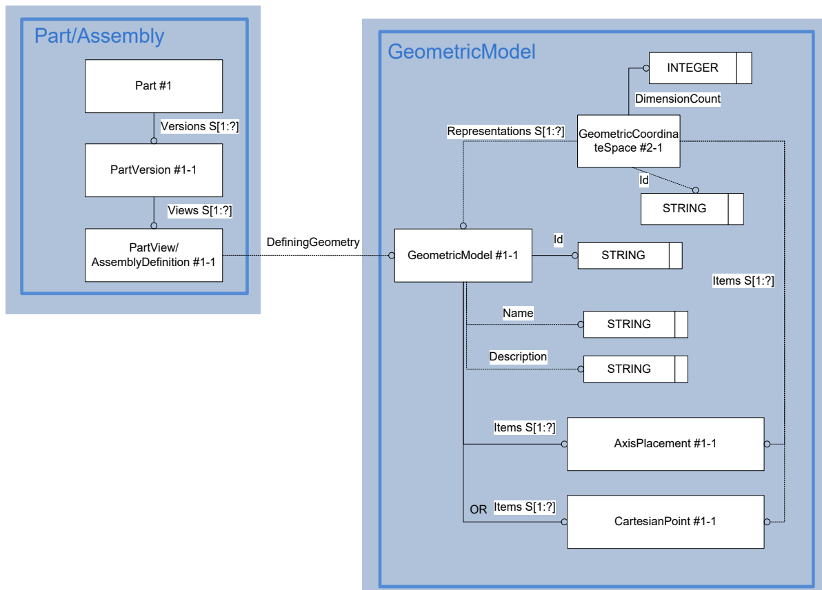
Figure 22: Template “GeometricModel”
