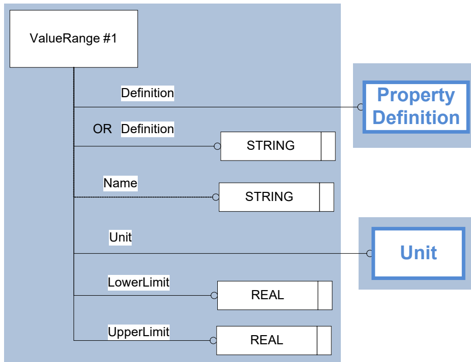
Figure 10: Template "ValueRange"
