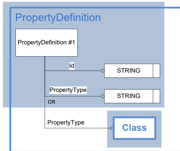
Figure 64: Template "PropertyDefinition"
