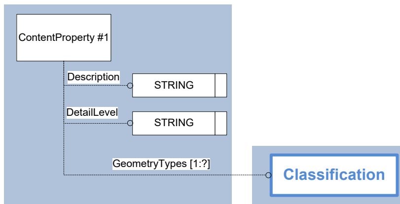
Figure 53: Template “ContentProperty”
