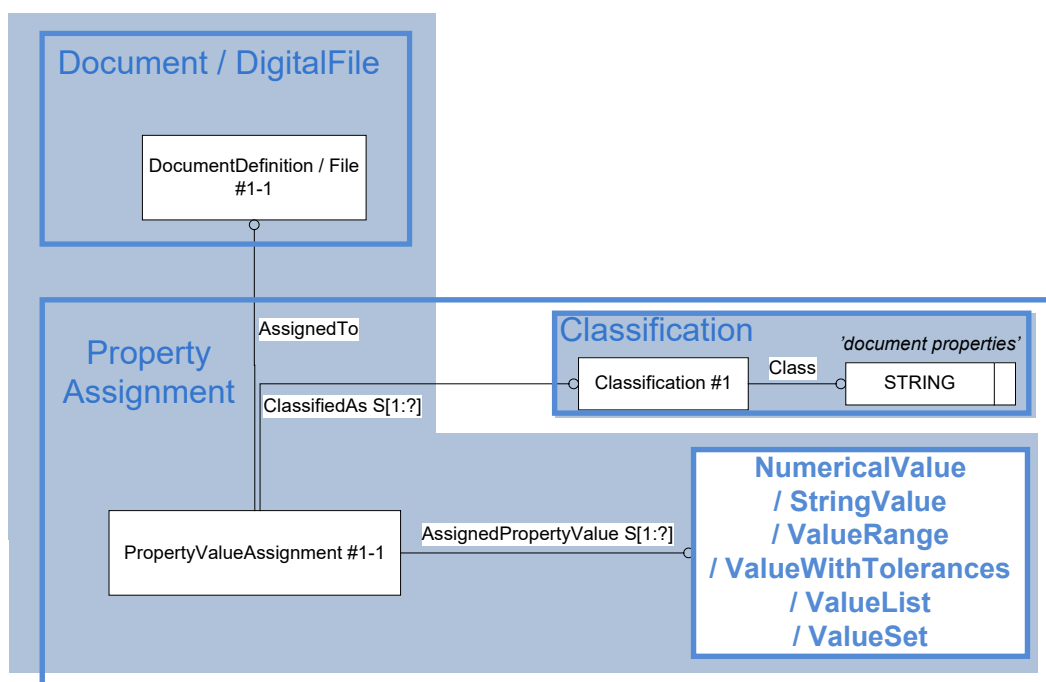
Figure 56: Template “DocumentFileProperty”
