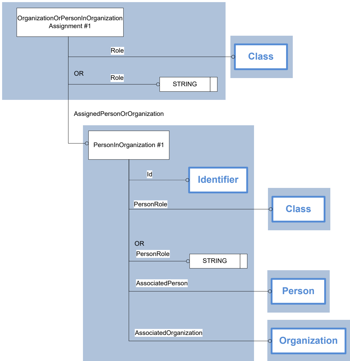
Figure 17: Template “PersonInOrganization”
