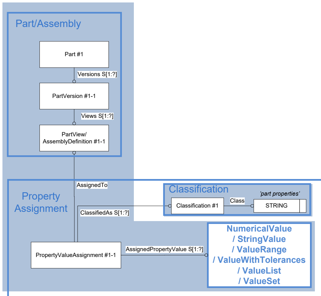
Figure 23: Template "PropertyAssignment"
