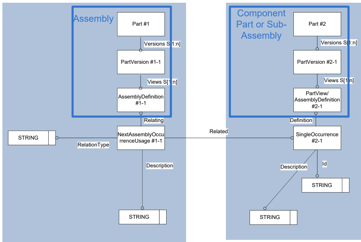
Figure 25: Template "SingleOccurrence"
