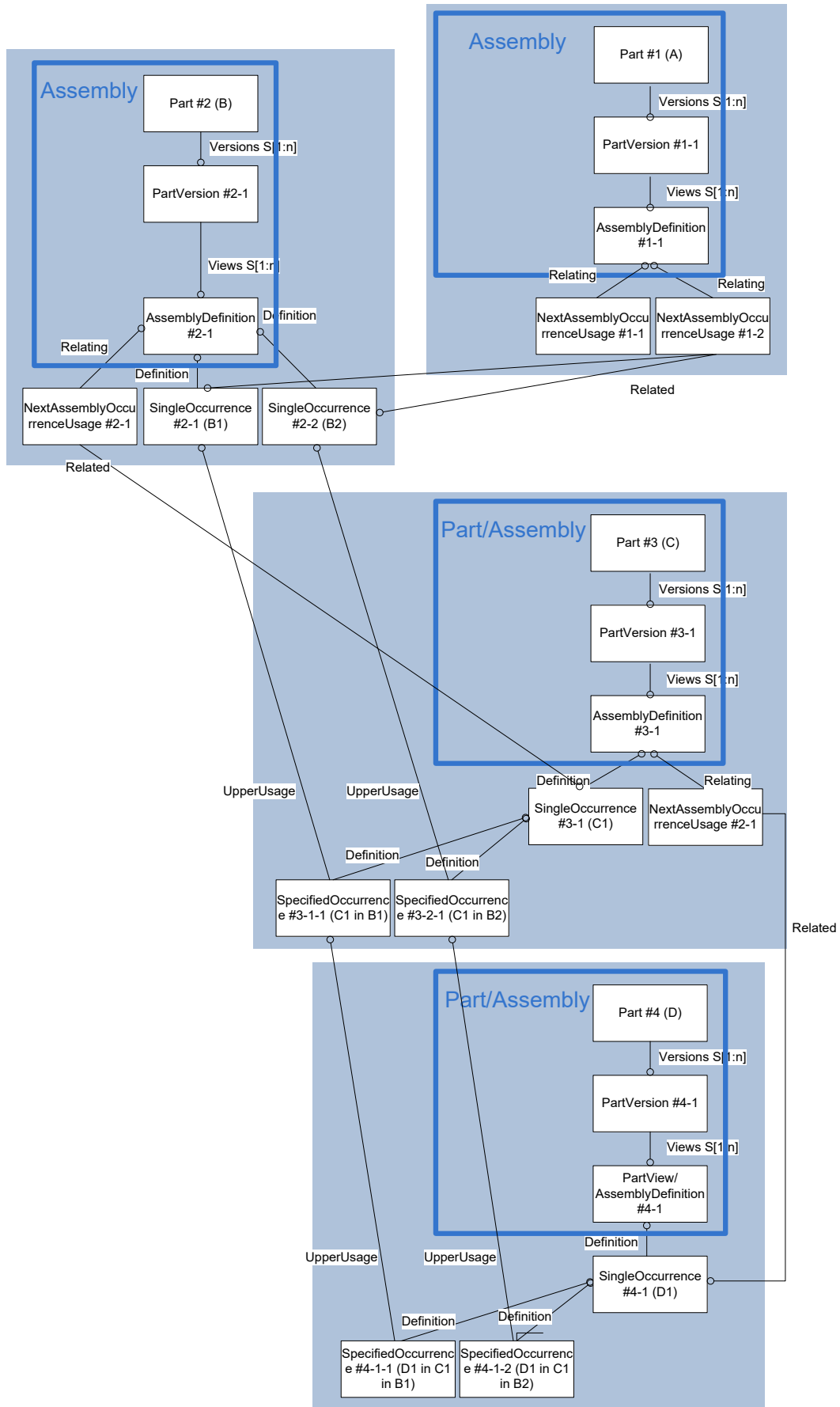
Figure 28: Template "SpecifiedOccurrence"
