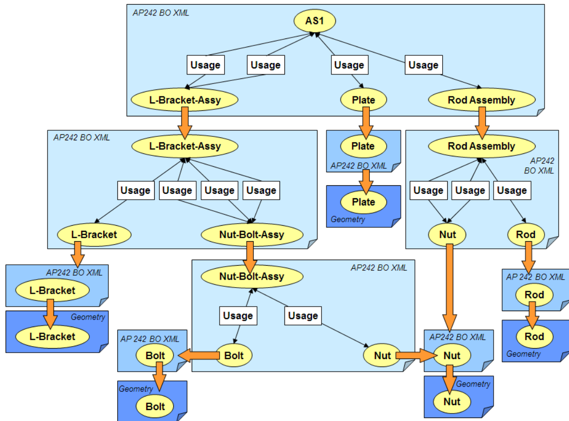
Figure 48: Example for Nested Structure with additional part-level XML files
