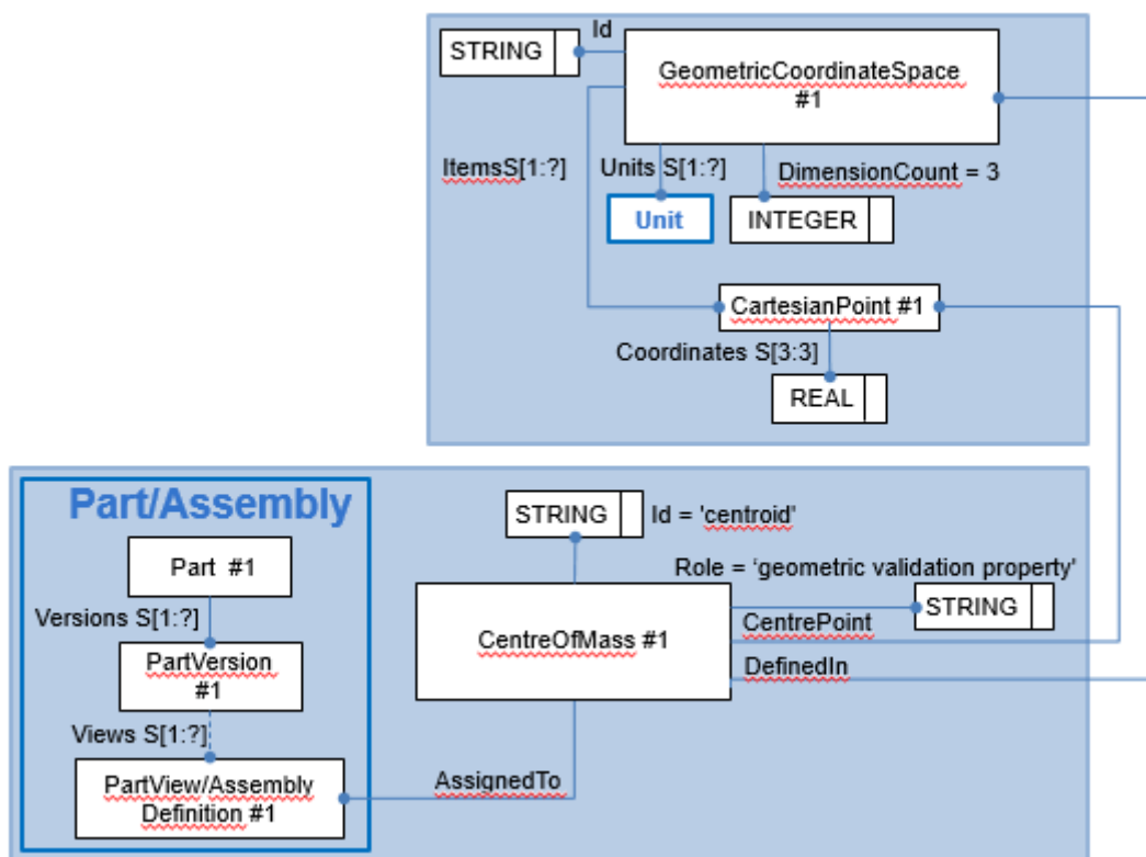
Figure 74: GVP 'centroid' or CentreOfMass assigned to a Part or Assembly
