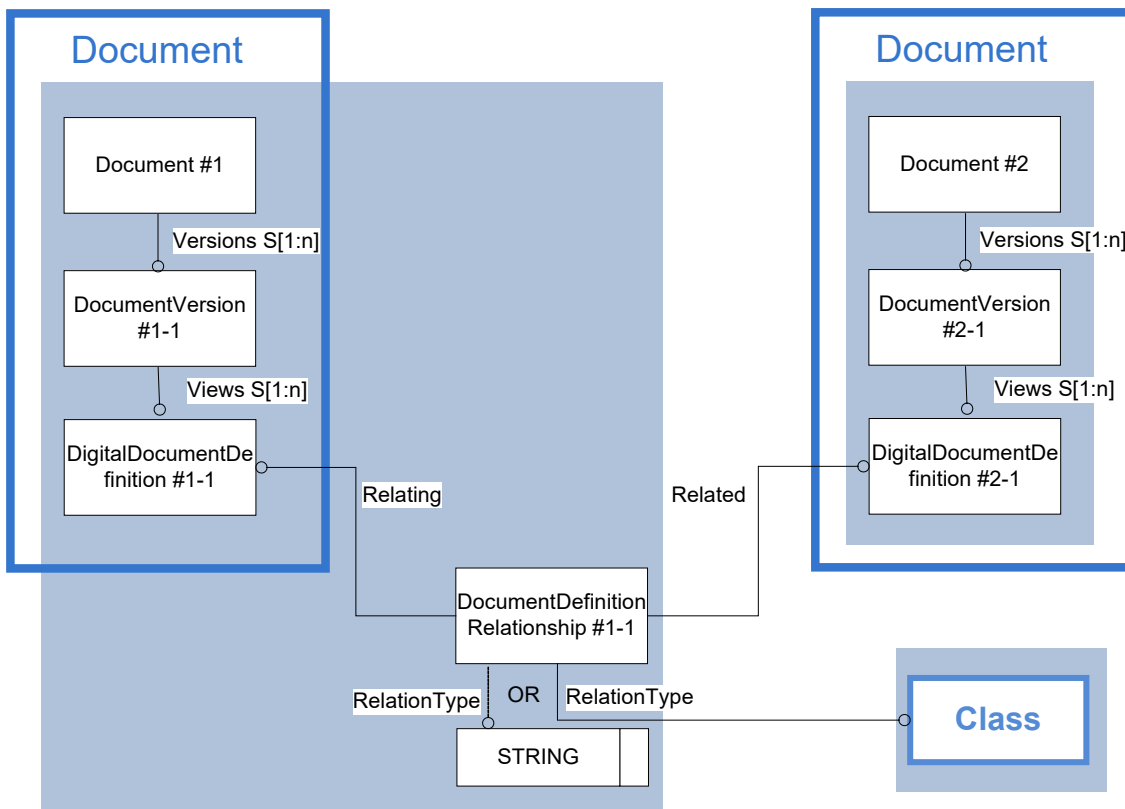
Figure 43: Template “DocumentDefinitionRelationship”
