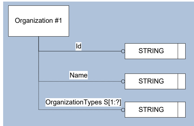
Figure 2: Template "Organization"
