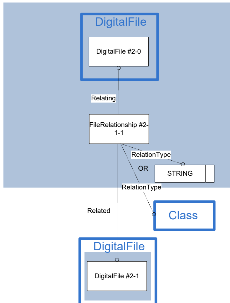
Figure 46: Template "FileRelationship"
