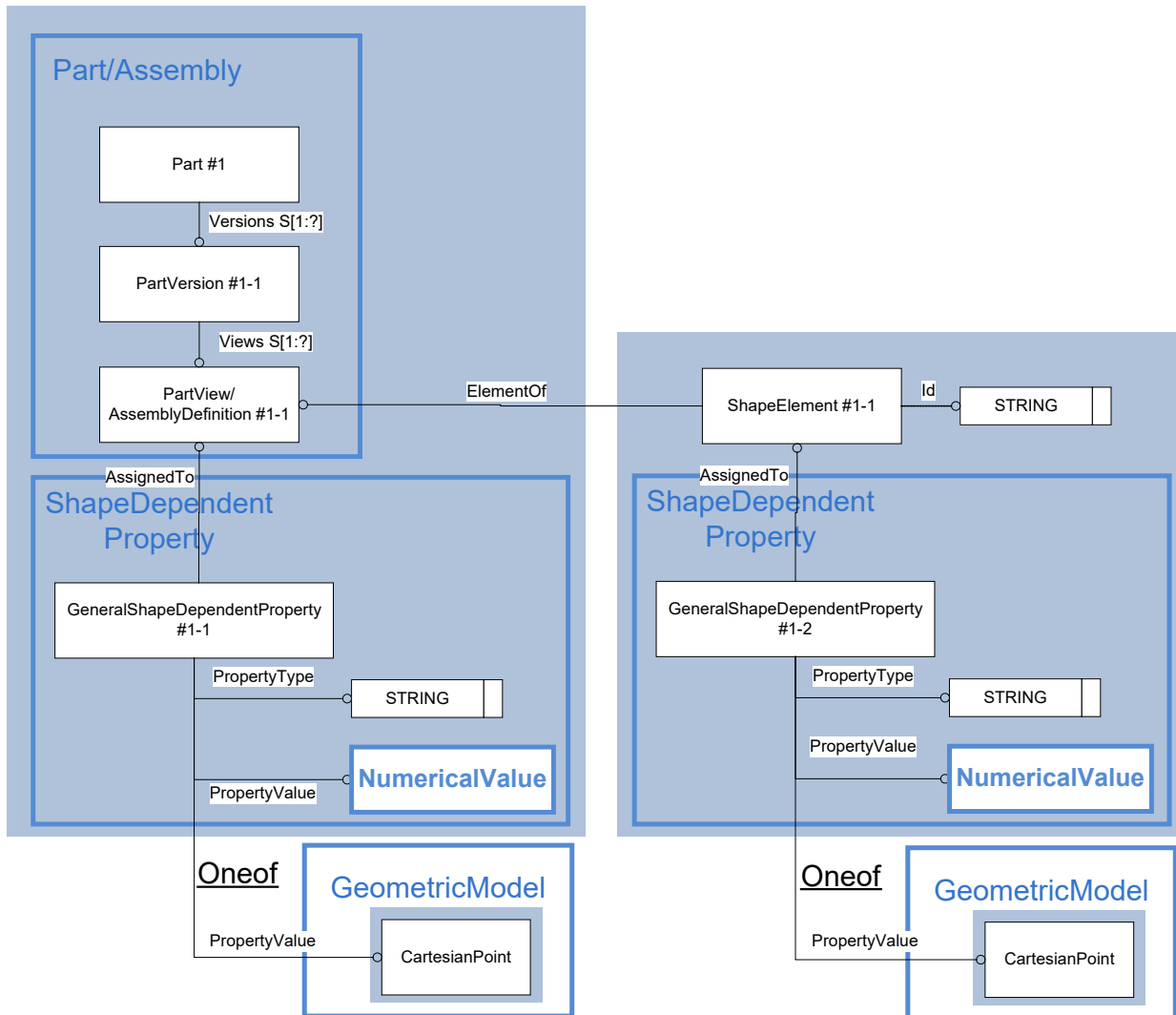
Figure 24: Template "ShapeDependentProperty" for either PartView or ShapeElement
