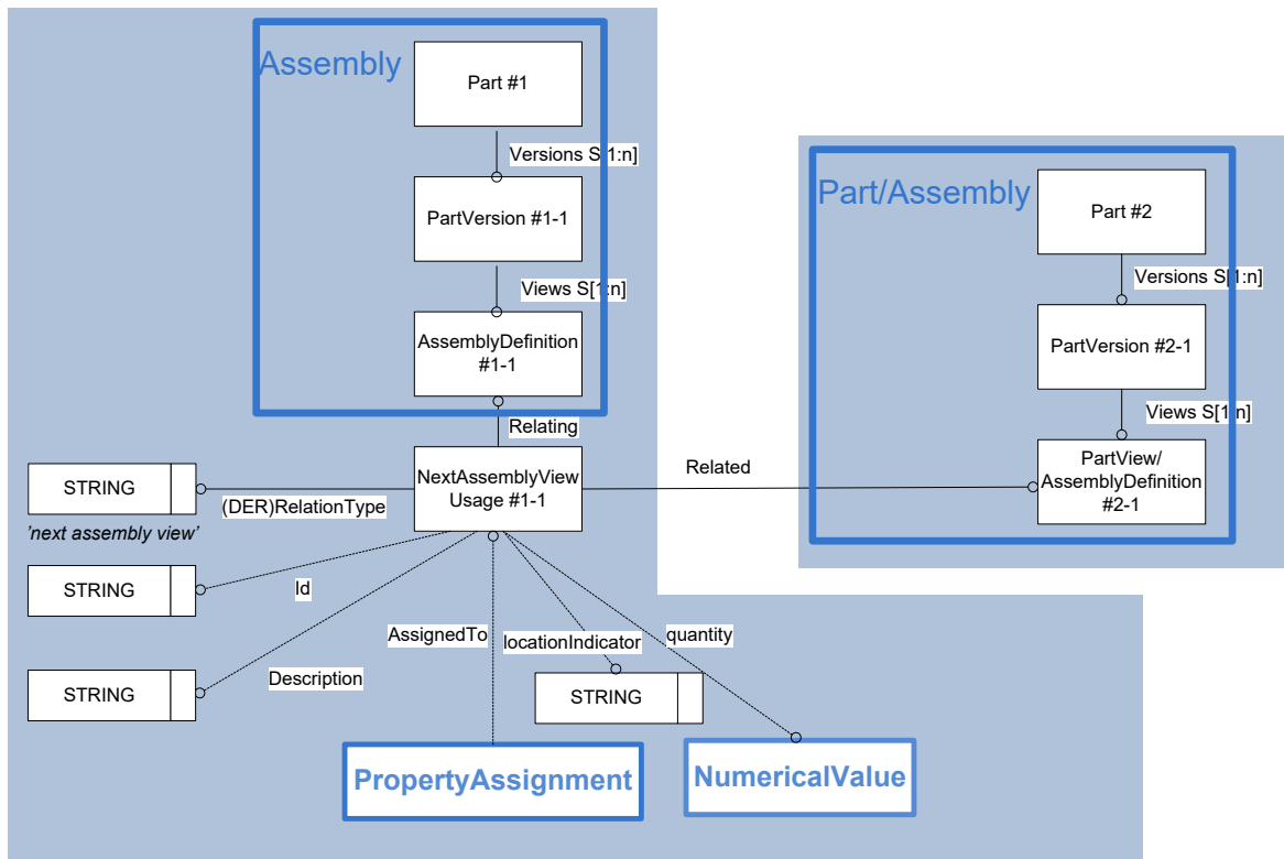
Figure 38: Template "PartViewRelationship" for quantity (+ properties)
