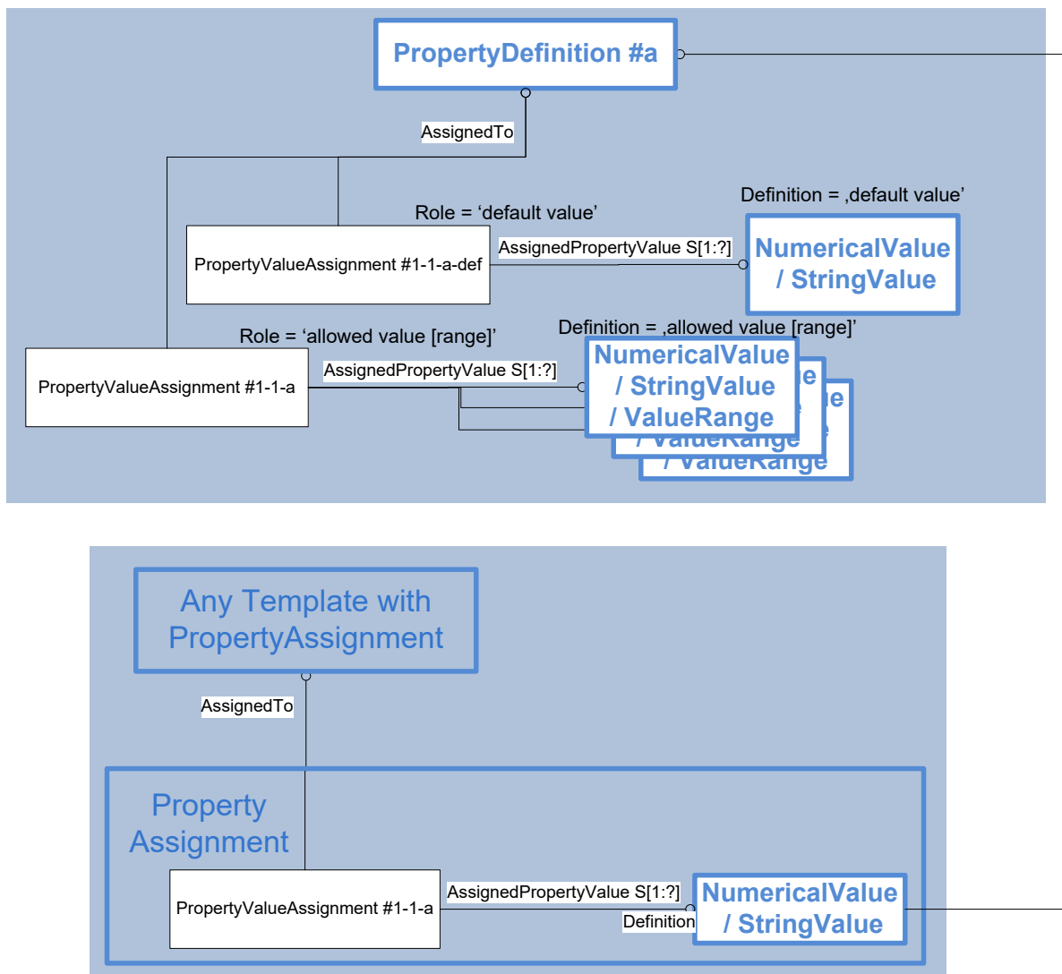
Figure 78: Default/Allowed values of customized properties
