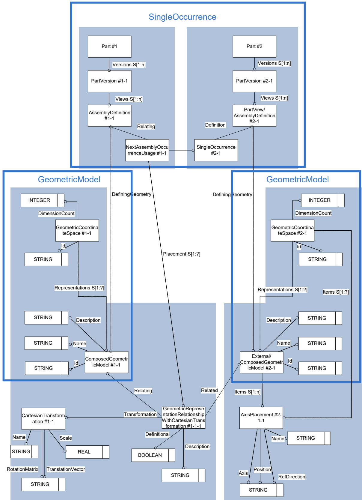
Figure 34: Full Positioning Representation with Explicit Transformation
