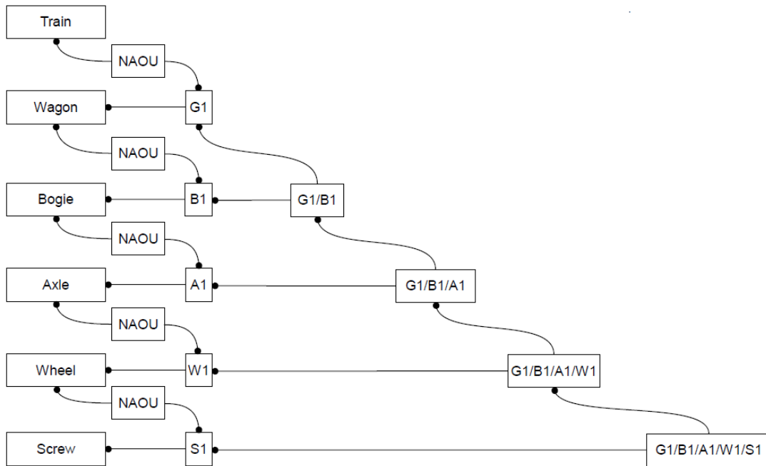
Figure 29: Instantiation without the intermediate SpecifiedOccurrences
