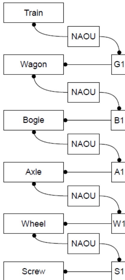
Figure 27: Example structure for multi-level assembly
