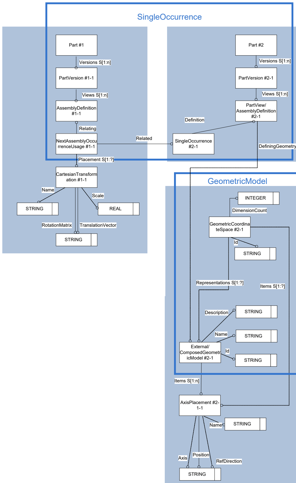
Figure 32: Instantiation example if Part #2 has geometry
