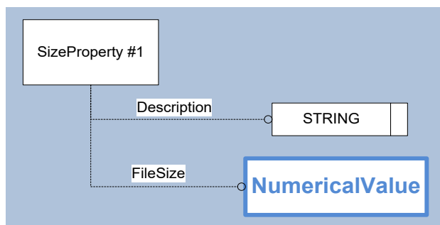
Figure 55: Template "SizeProperty"
