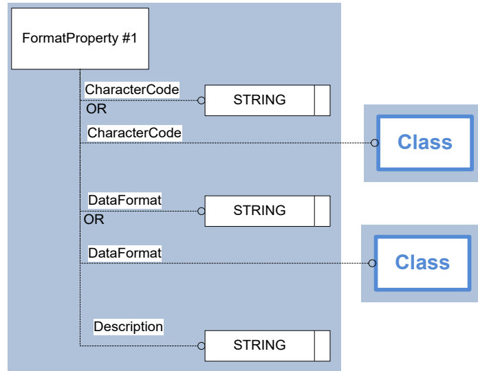
Figure 52: Template “FormatProperty”
