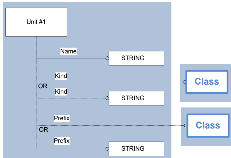
Figure 3: Template “Unit”
