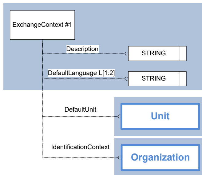
Figure 1: Template “ExchangeContext”
