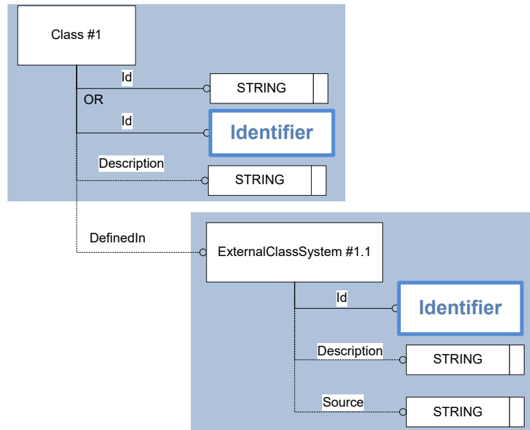
Figure 4: Template "Class"
