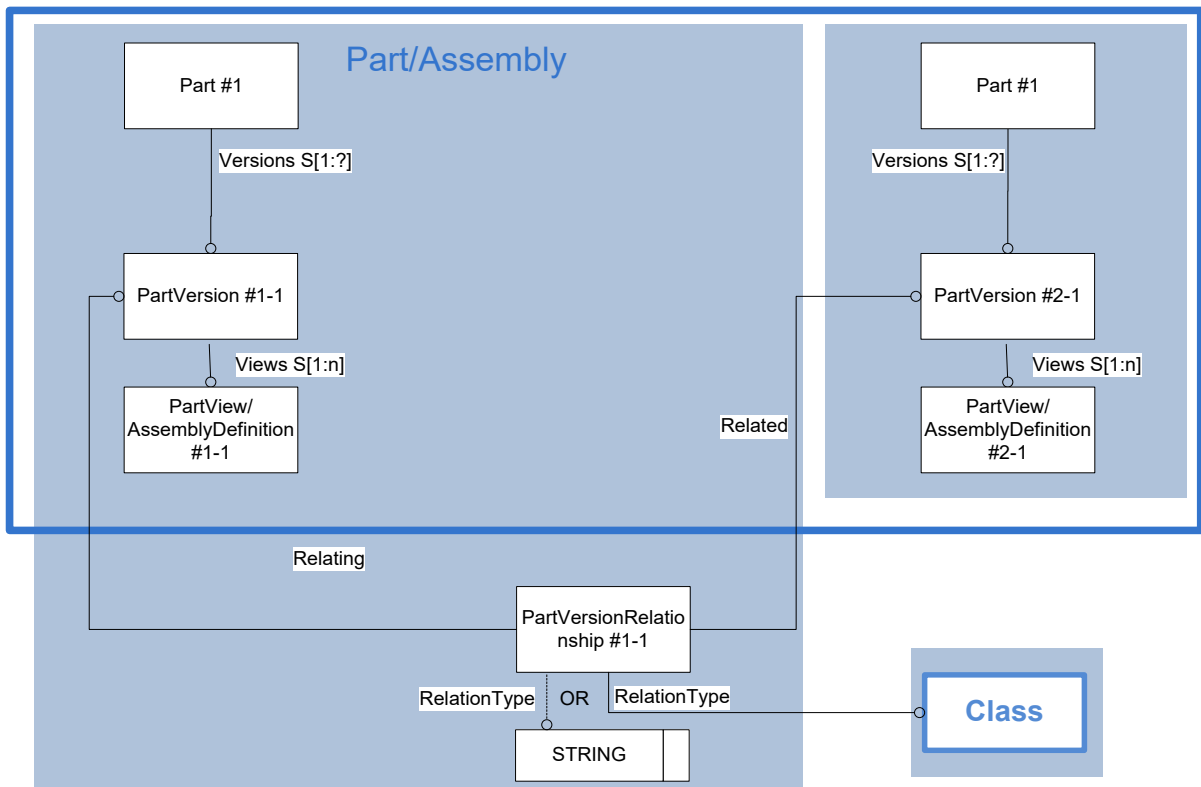
Figure 21: Template "PartVersionRelationship"
