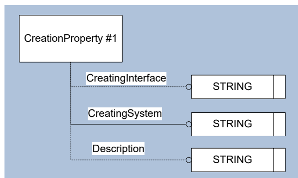
Figure 54: Template “CreationProperty”
