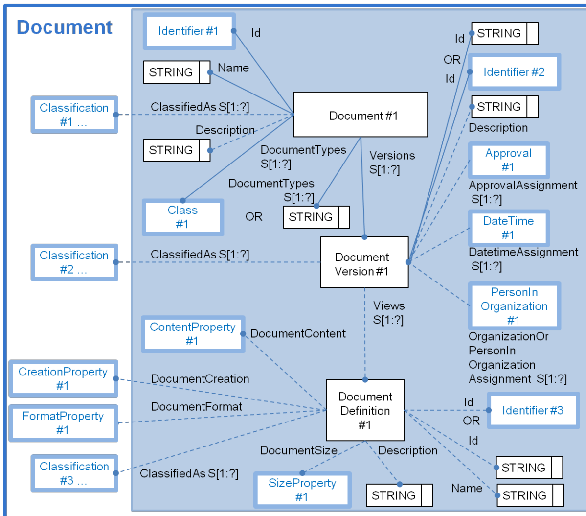
Figure 42: Template “Document”
