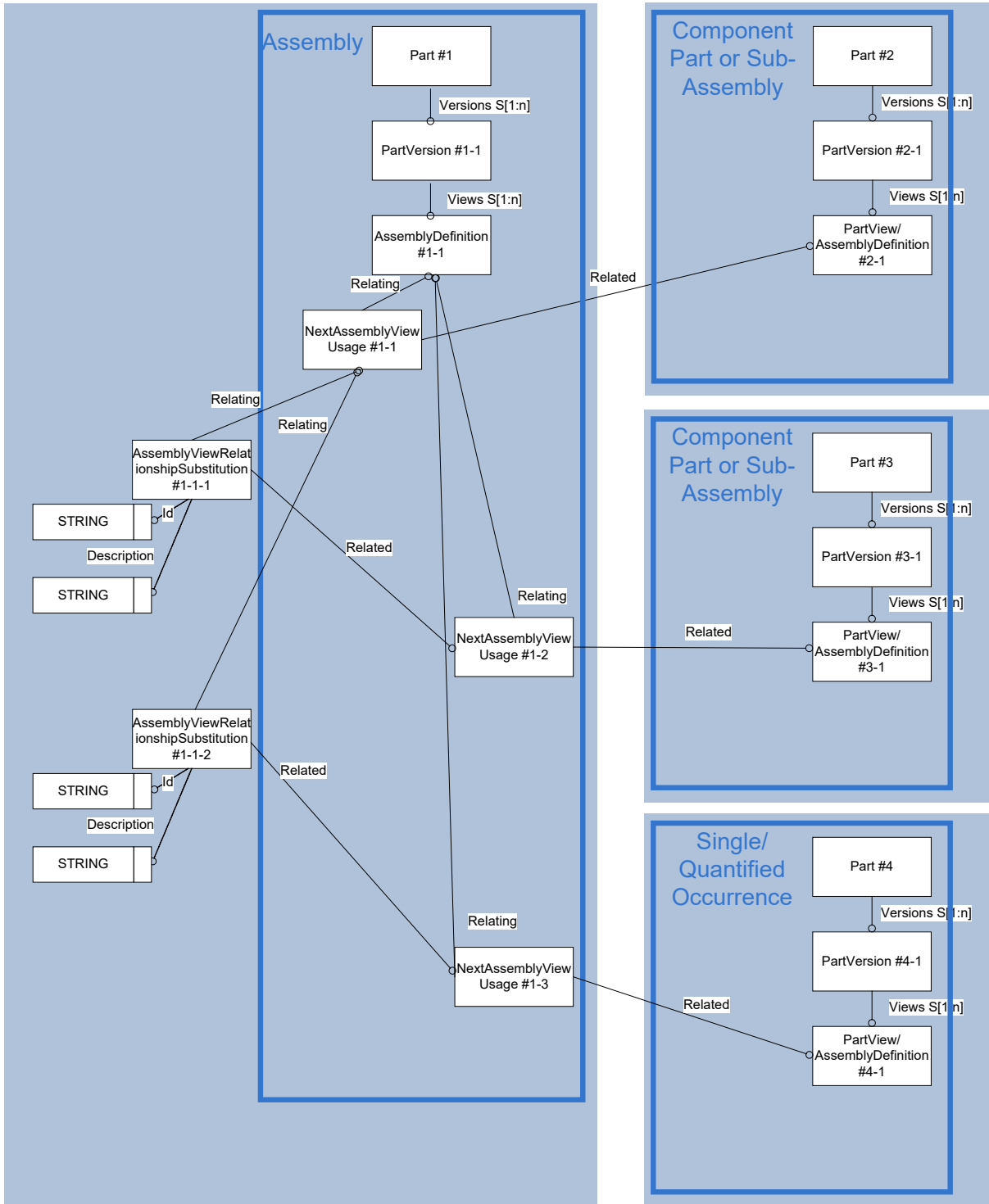
Figure 41: Template "AssemblyViewRelationshipSubstitution"
