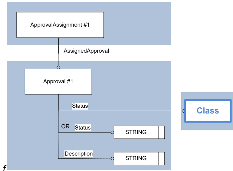
Figure 15: Template “Approval”
