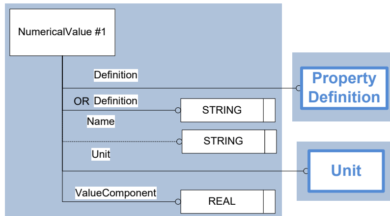
Figure 8: Template "NumericalValue"
