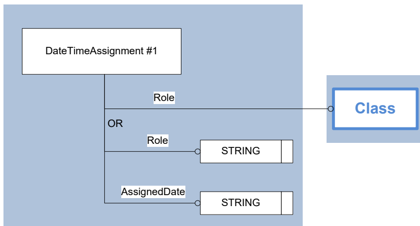
Figure 14: Template "DateTime"
