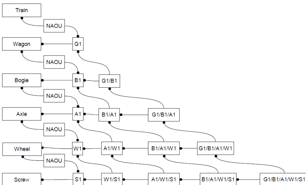
Figure 30: Instantiation with all the intermediate SpecifiedOccurrences
