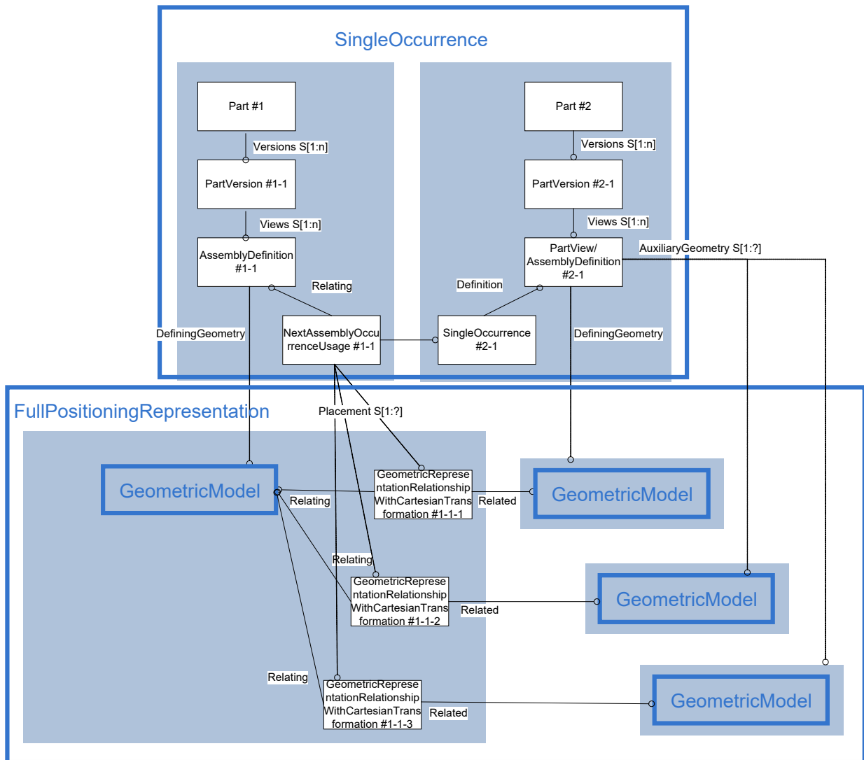
Figure 26: Cross-reference of Defining/Auxiliary Geometry and NextAssemblyOccurrenceUsage.Placement
