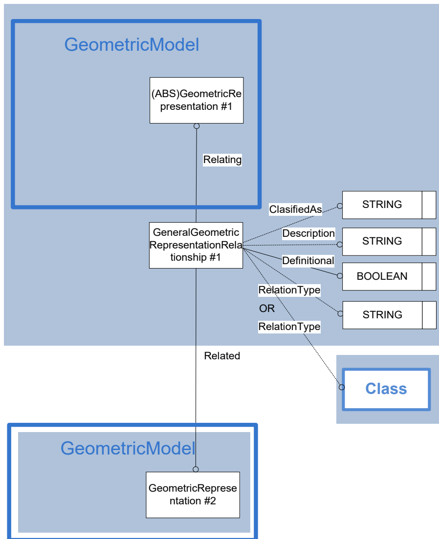
Figure 36: General Geometric Representation Relationship
