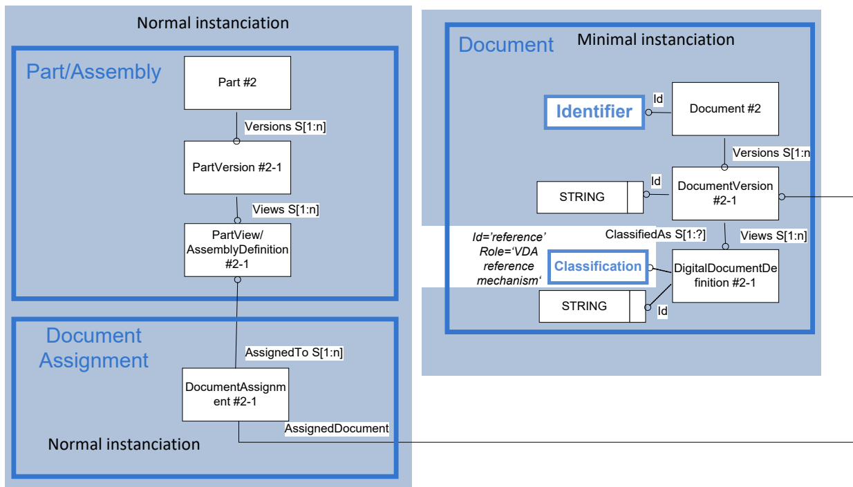
Figure 51: Template “Document reference”
