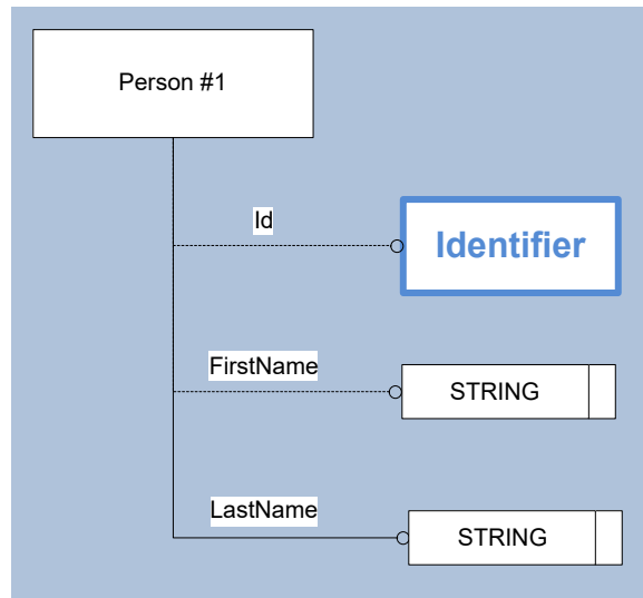
Figure 16: Template “Person”
