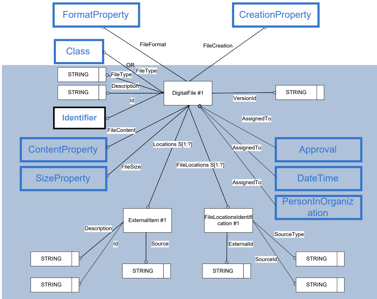
Figure 45: Template "DigitalFile"
