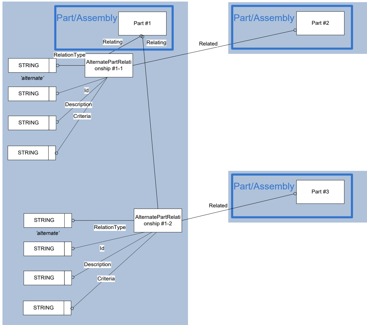
Figure 39: Template "AlternatePartRelationship"
