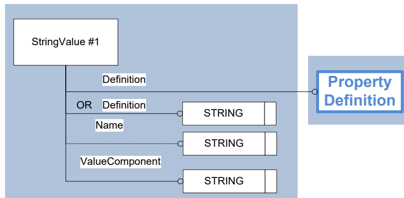
Figure 9: Template “StringValue”
