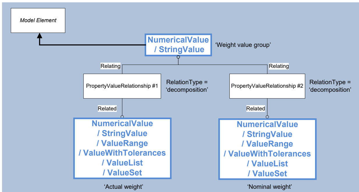
Figure 65: Defining a group of attribute values
