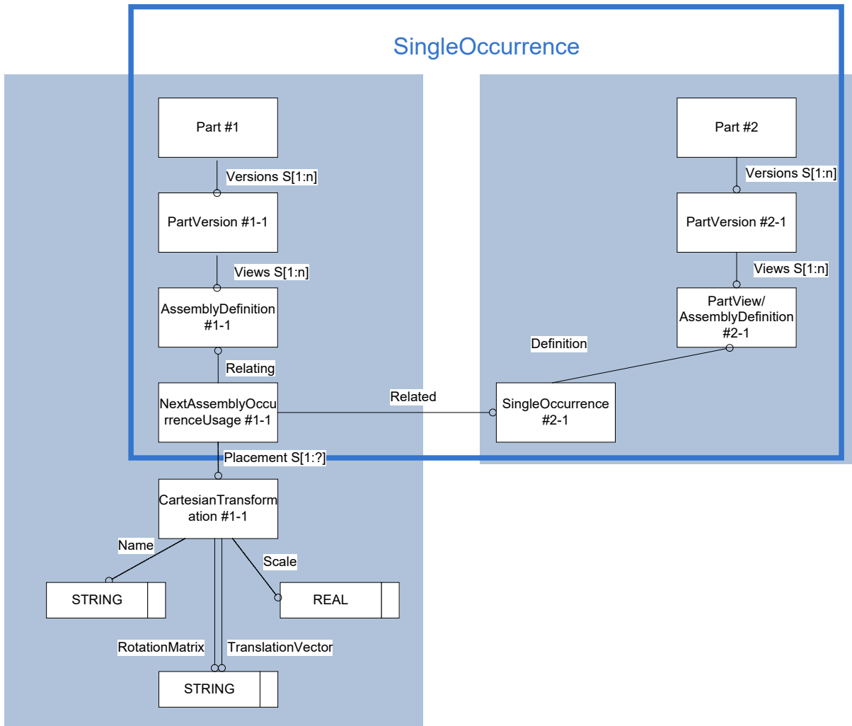
Figure 31: Template "Simplified Positioning Representation"
