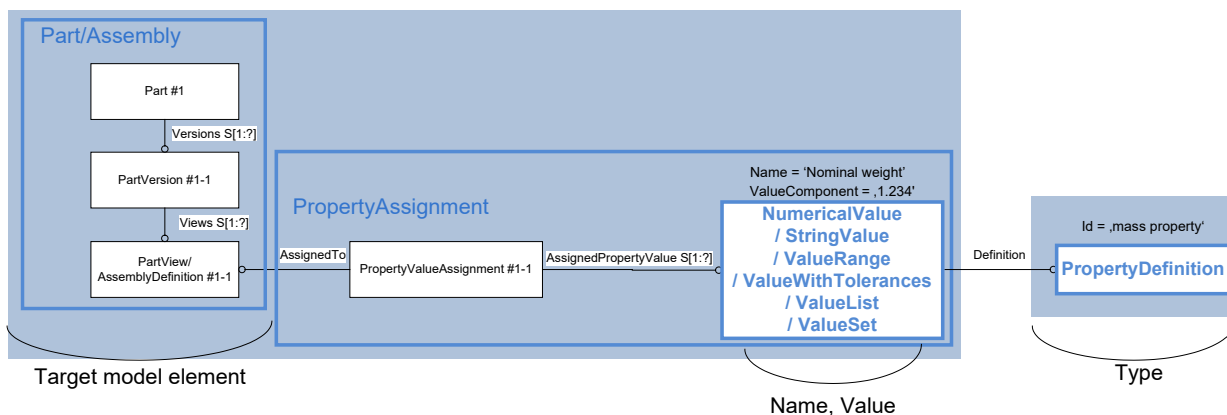
Figure 66: User defined attribute at the part/assembly level
