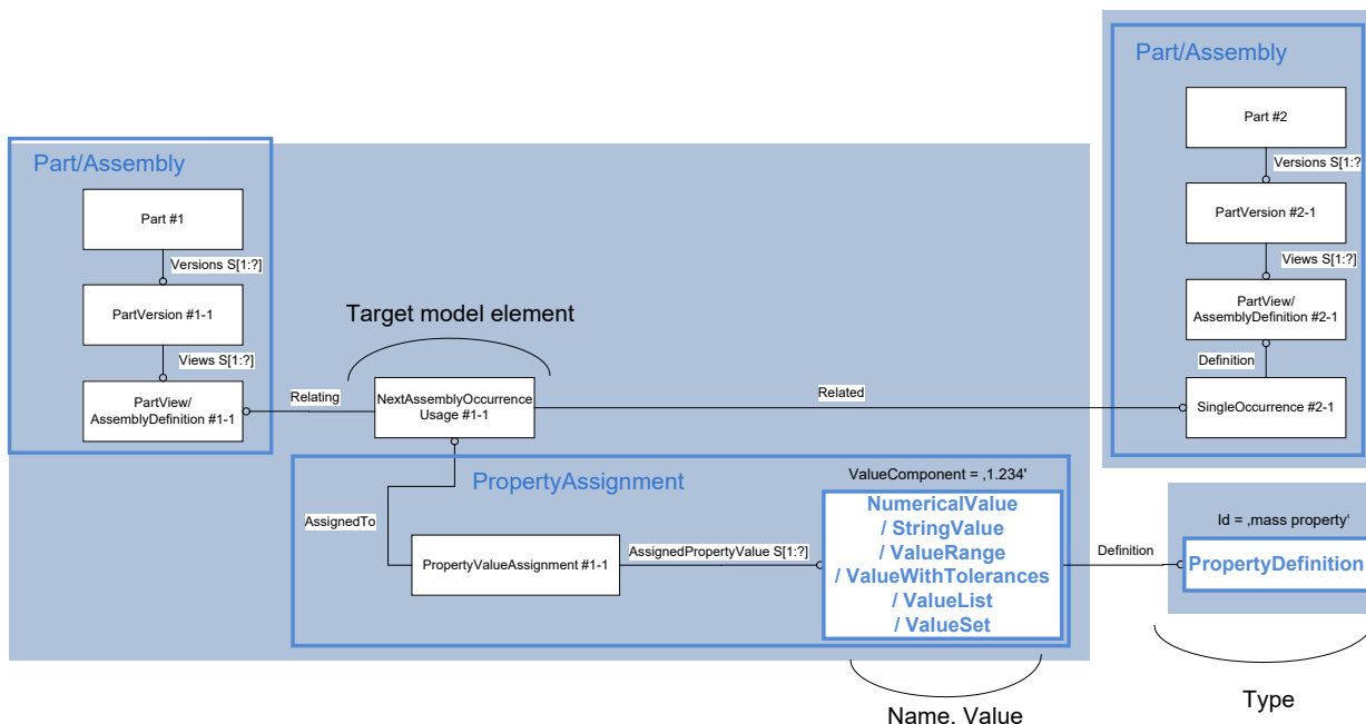
Figure 67: User defined attribute for a simple component instance in an assembly
