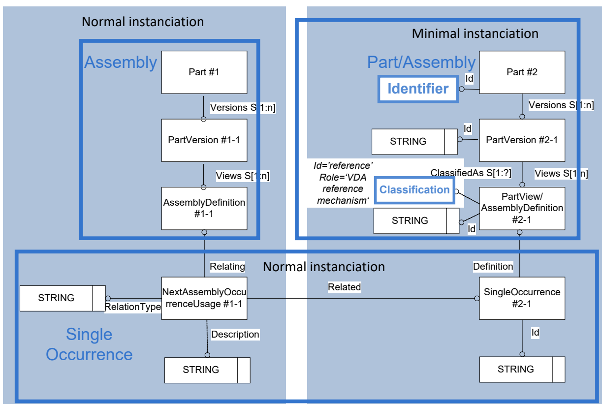
Figure 50: Template "Component reference"
