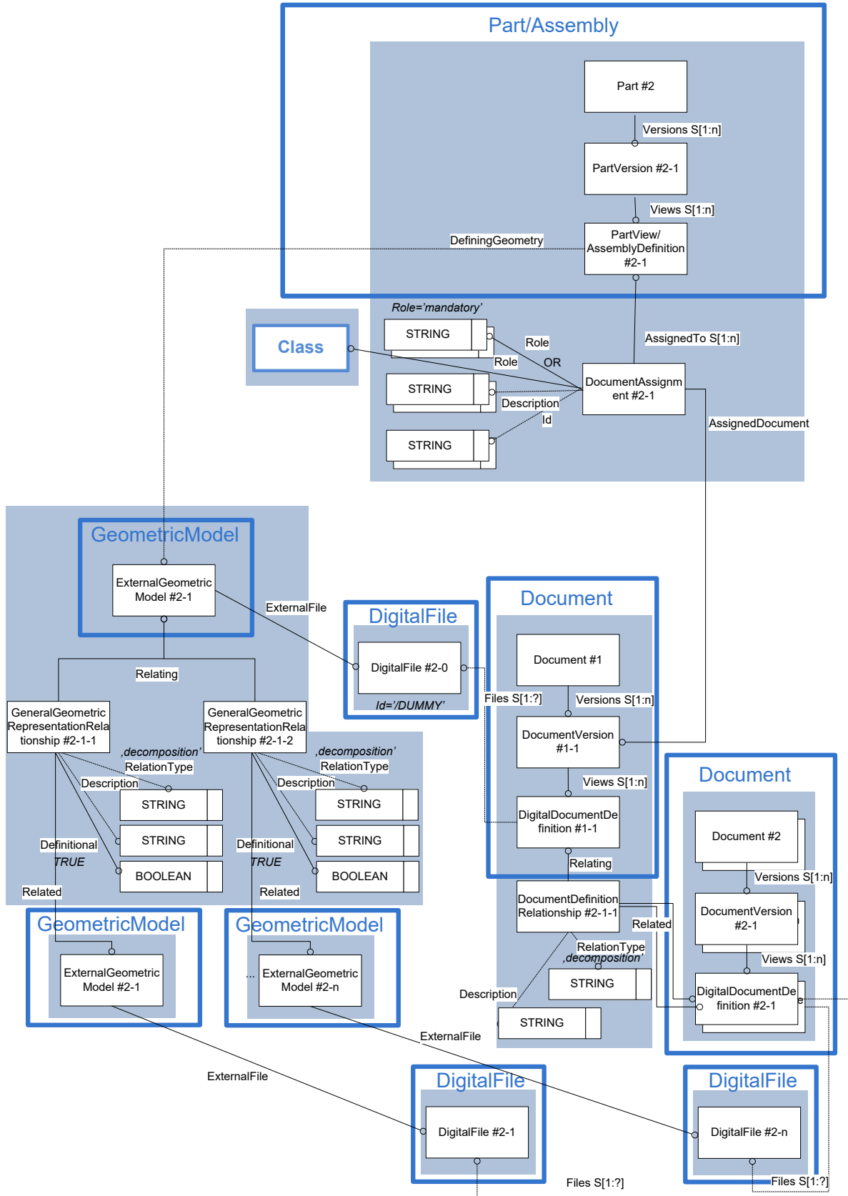
Figure 61: Model splitting for "PDM Representation for DocumentAssignment"
