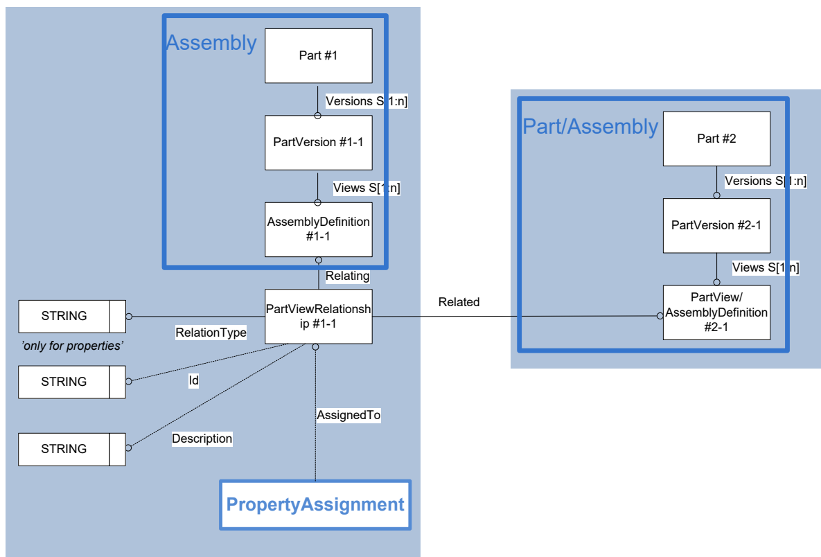
Figure 37: Template "PartViewRelationship" for properties
