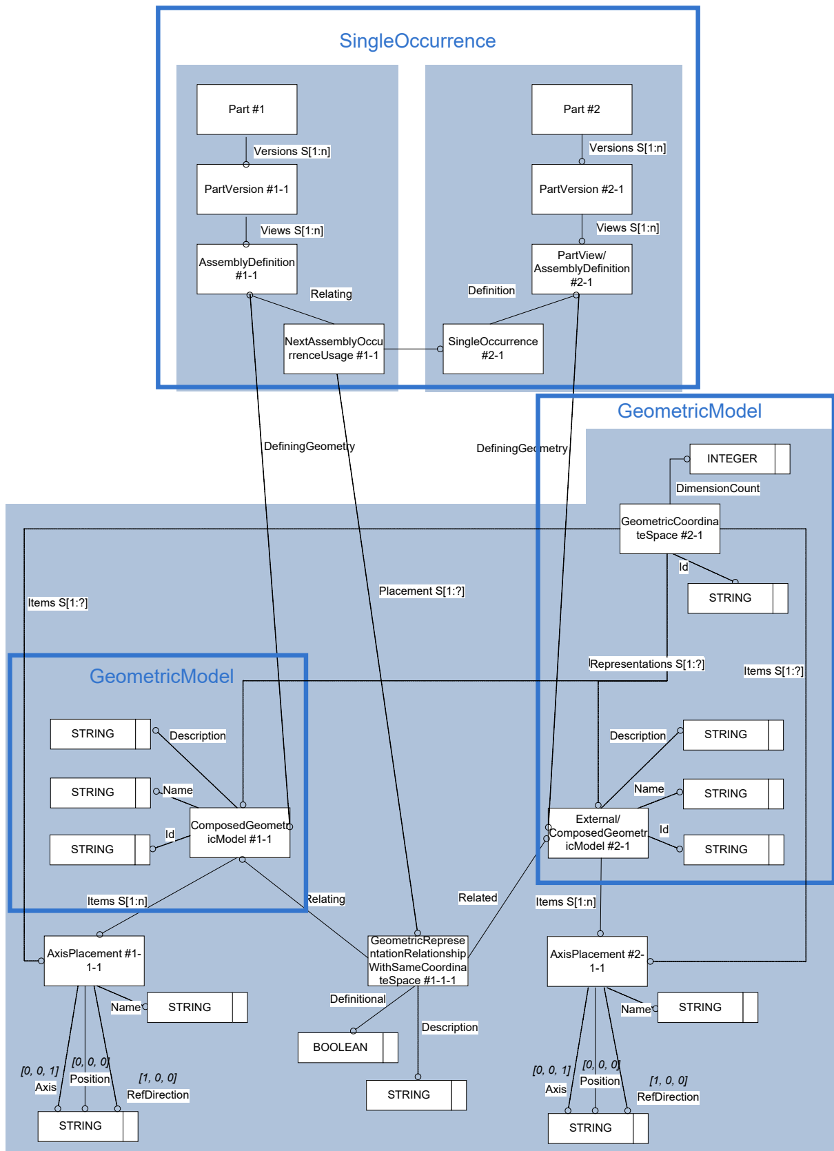
Figure 35: Full Positioning Representation with Same Coordinate Space
