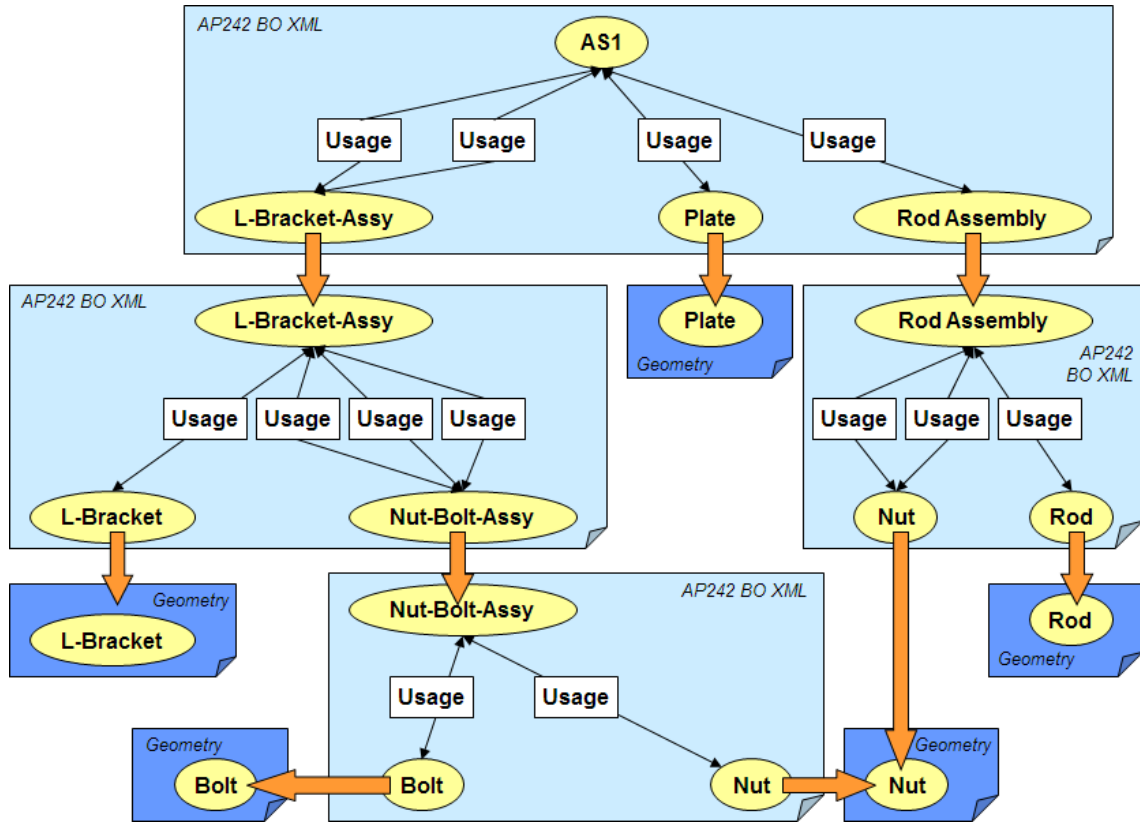
Figure 47: Example for Nested Structure
