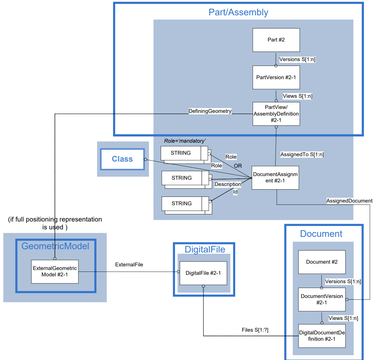
Figure 60: Template "PDM Representation for DocumentAssignment"
