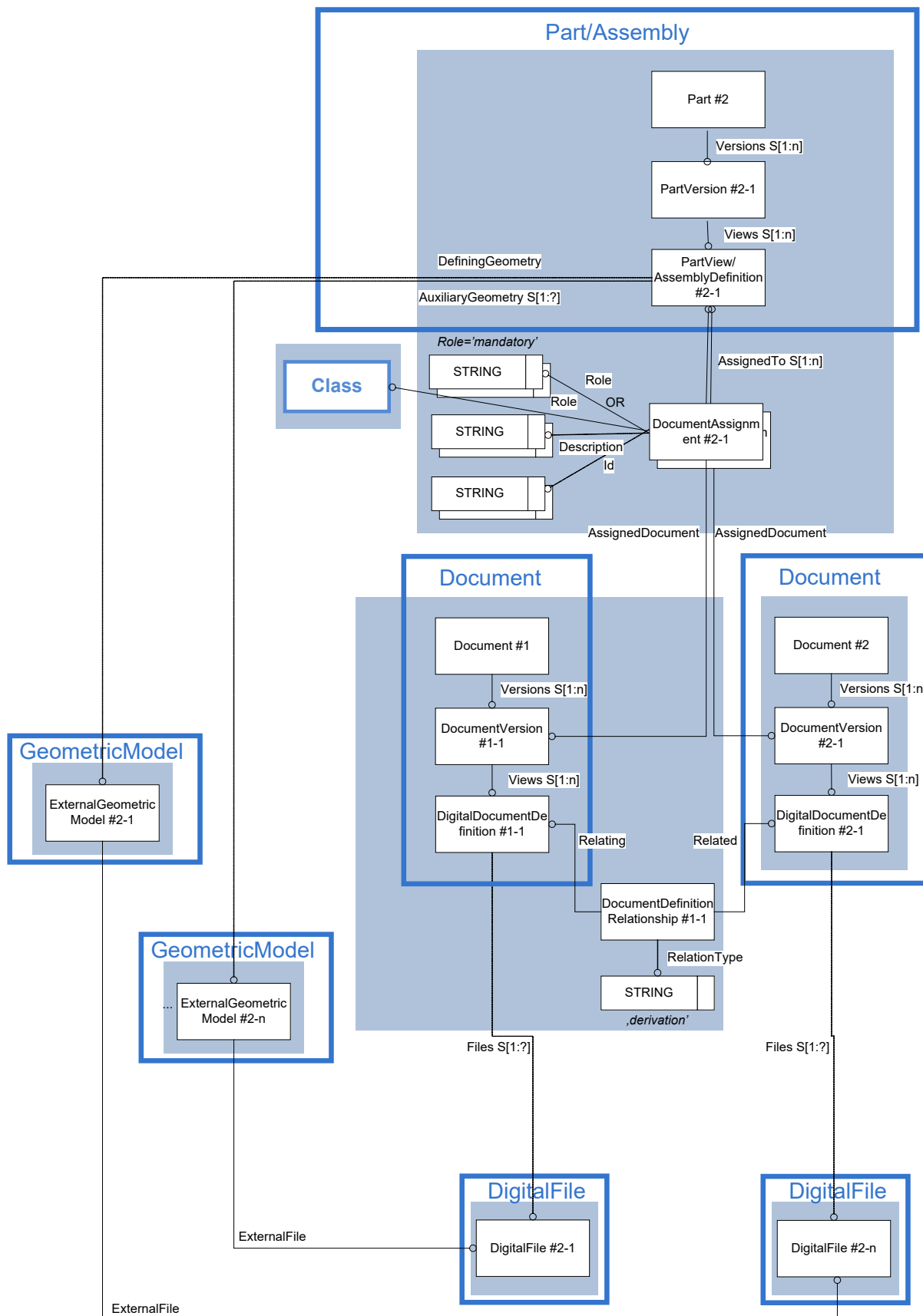
Figure 62: Alternate models for "PDM Representation for DocumentAssignment"
