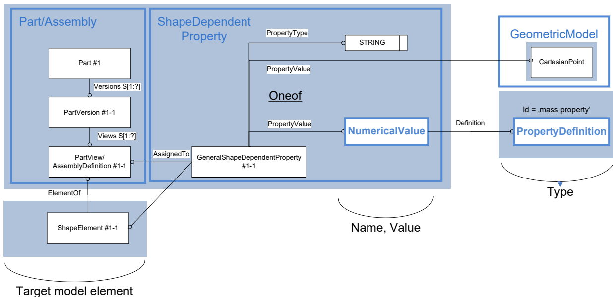
Figure 68: User defined attribute for a shape or a portion of shape
