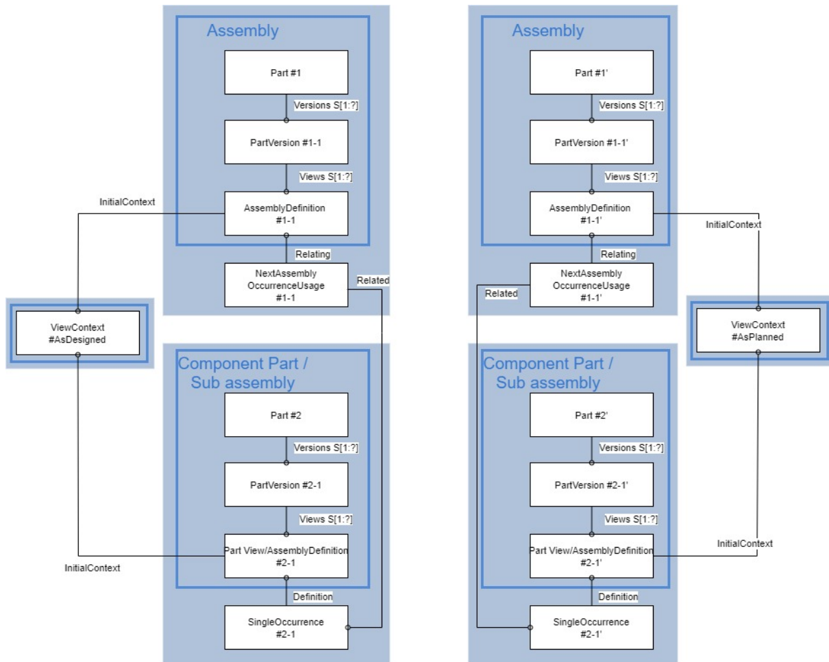
Figure 79: Representation of As Designed and As Planned views
