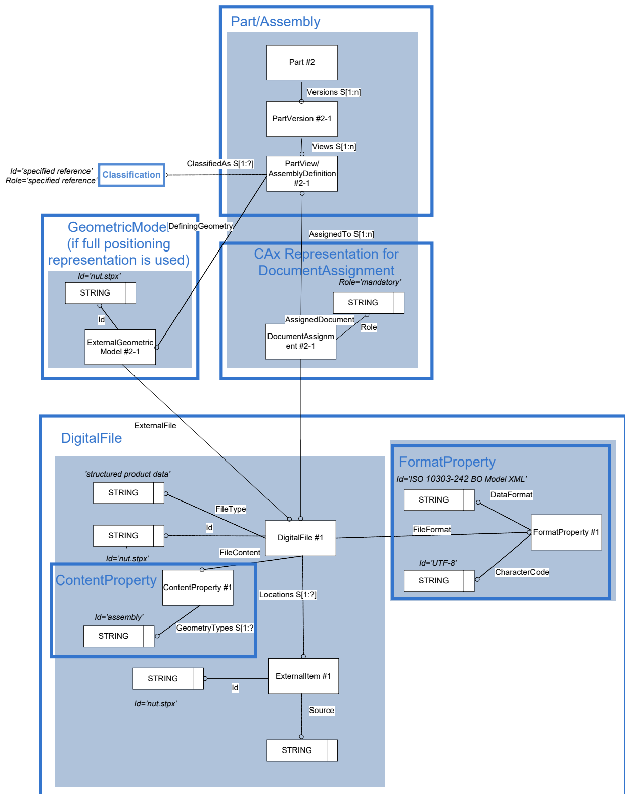
Figure 49: Element Structure for Nested XML File
