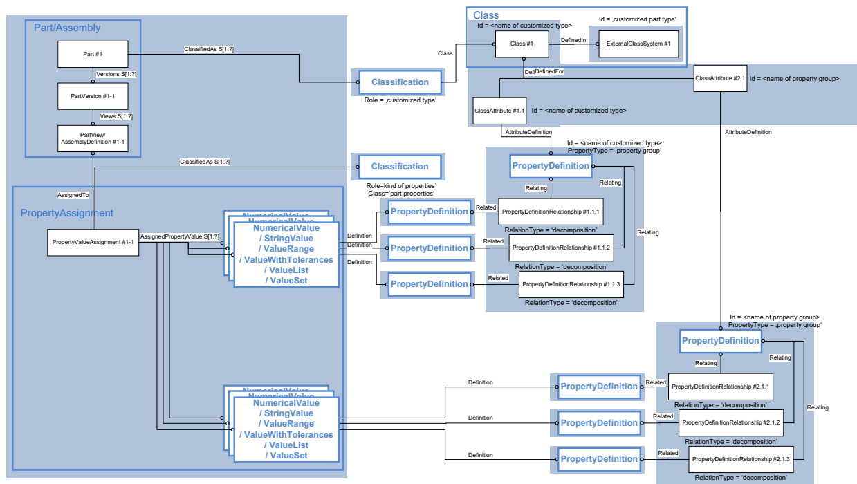
Figure 77: Example of property groups on a Part having properties on the PartView.
