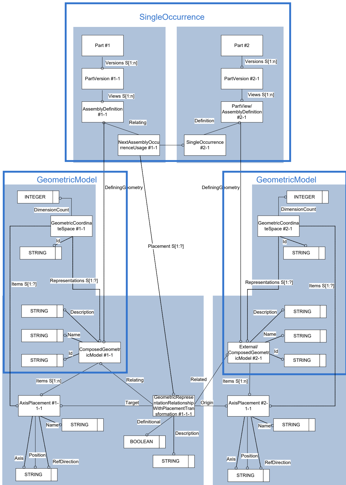
Figure 33: Full Positioning Representation with Implicit Transformation
