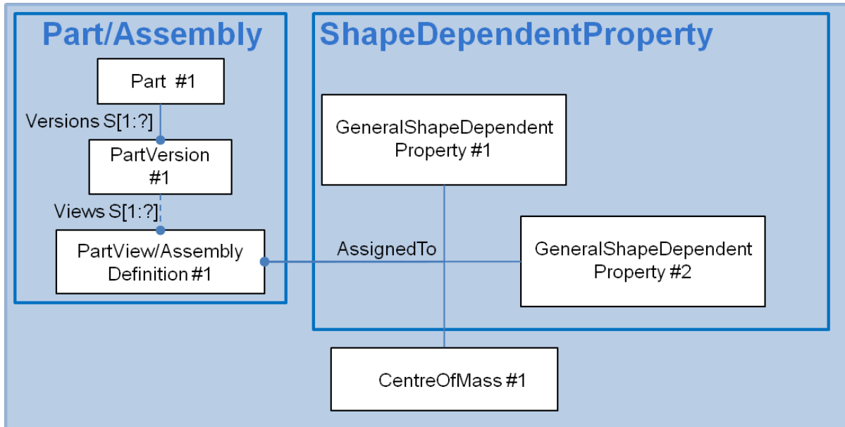
Figure 71: Geometric Validation Properties at the Part and Assembly level
