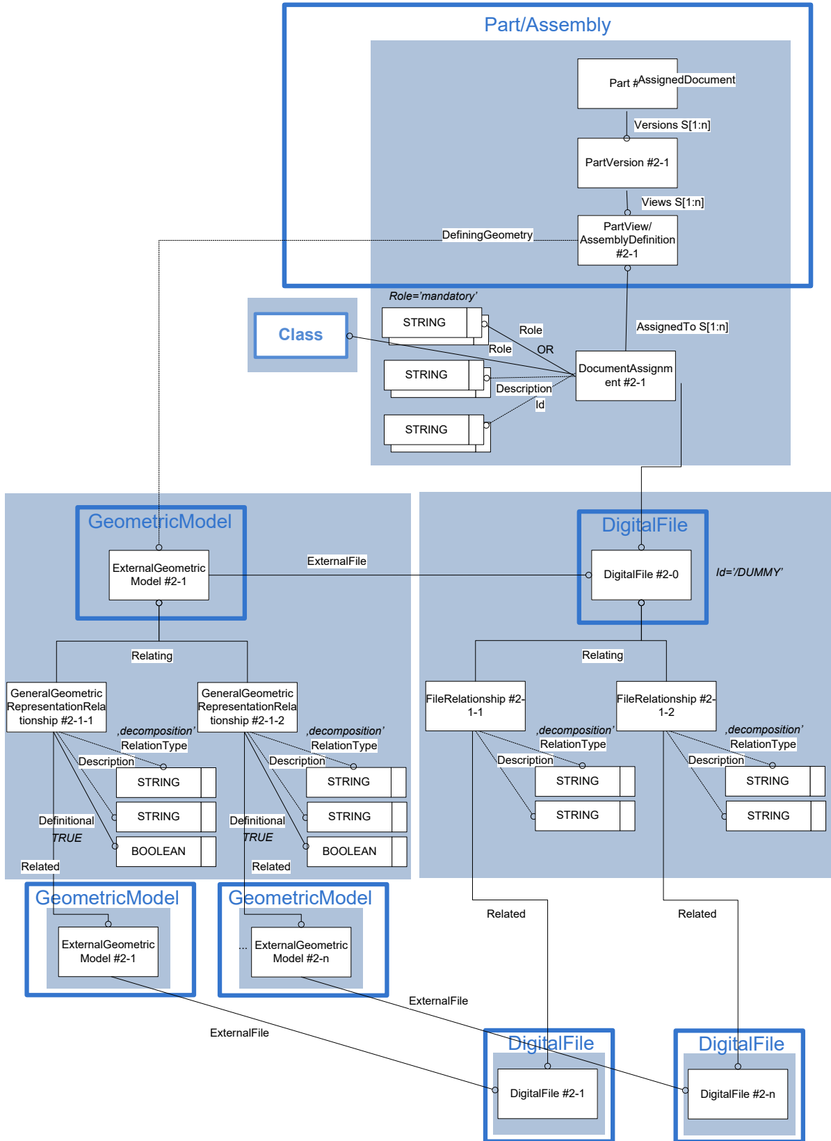
Figure 58: Model splitting for "CAx Representation for DocumentAssignment"
