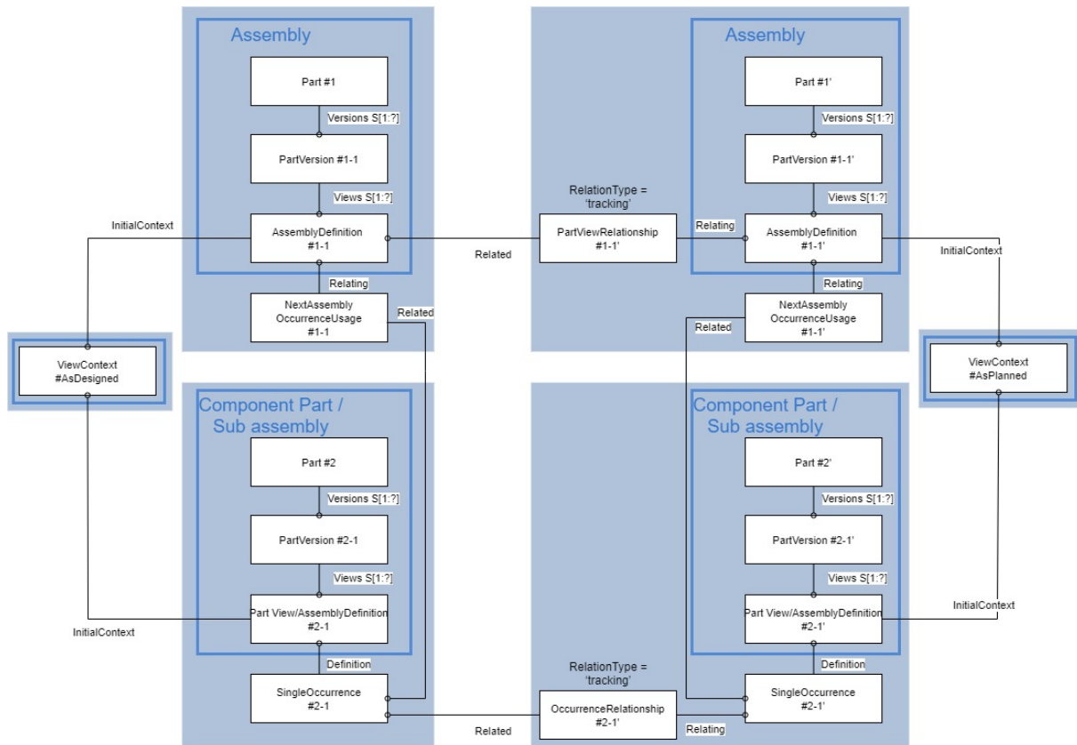
Figure 80: Representation of tracking relationship
