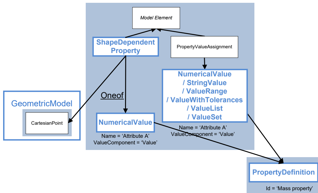
Figure 63: Definition of an attribute name and its usage
