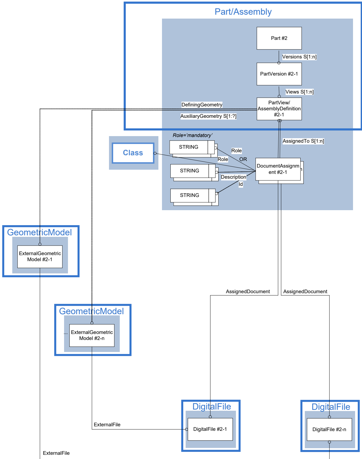
Figure 59: Alternate models for "CAx Representation for DocumentAssignment"
