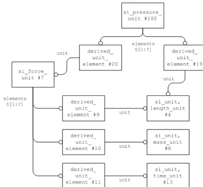
Figure 15: SI Unit Definition for "Pascal"
