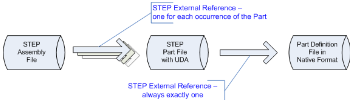
Figure 13: Intermediate File for External References with Part-Level UDA
