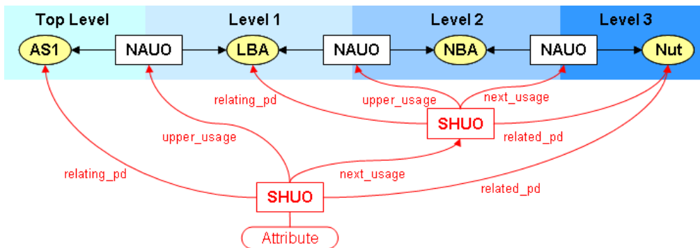
Figure 6: Use of multiple SHUOs to navigate through the assembly structure
