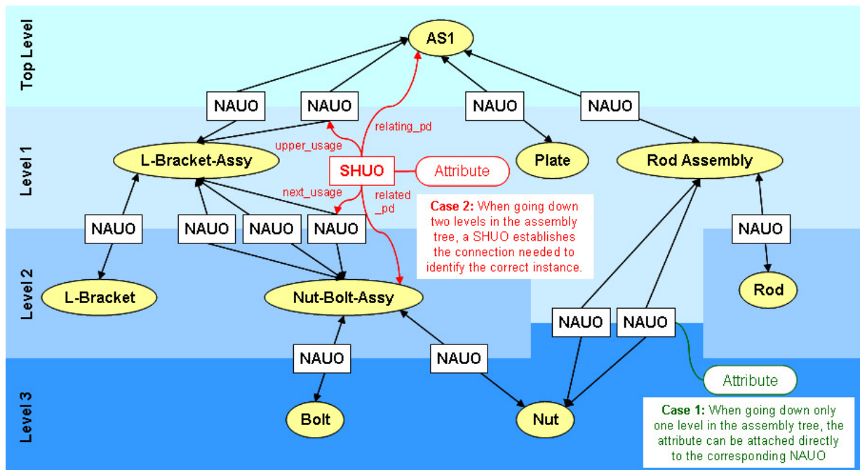
Figure 5: The use of SHUO to identify an instance deeper down in the assembly
