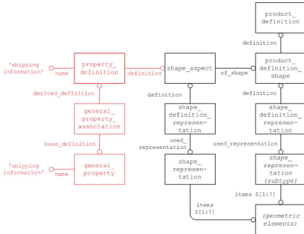
Figure 7: Assignment of an attribute at the solid/surface level
