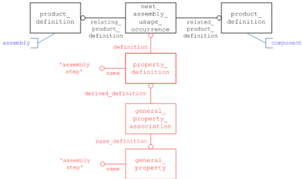
Figure 4: User defined attribute for a simple component instance in an assembly
