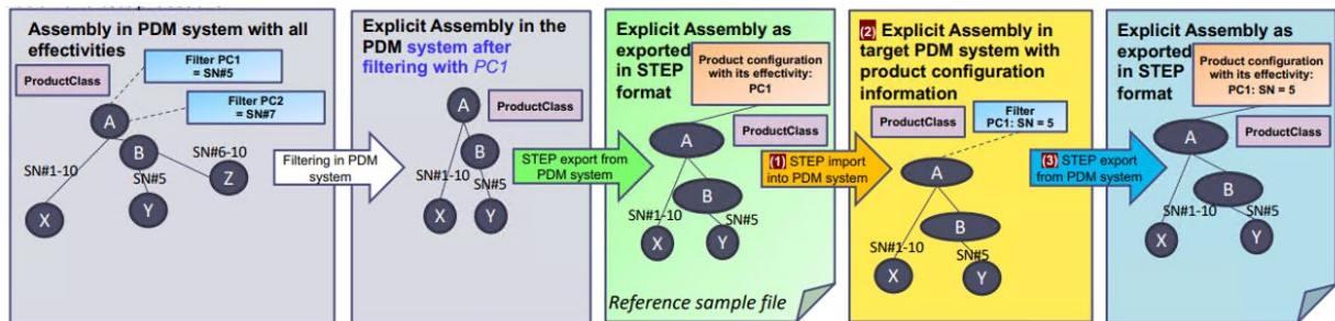
Figure 41: Example for overall process overview for Export of effectivity based single product configuration as explicit assembly structure with effectivities
