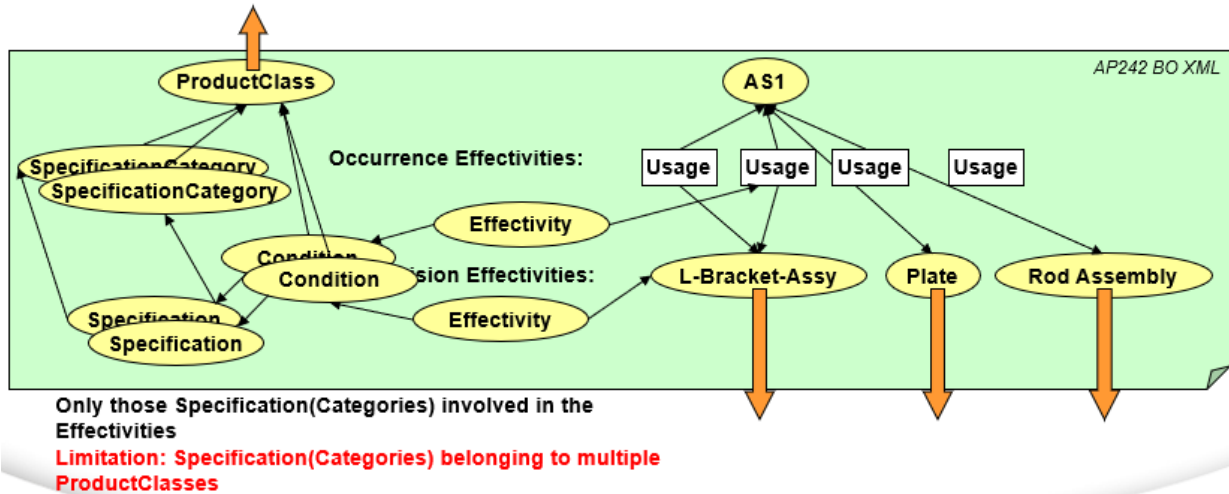
Figure 48: Example for Nested Structure with Effectivities making only use of Specifications
