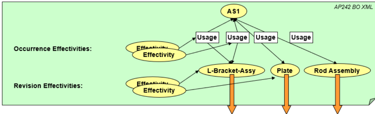
Figure 45: Example for Nested Structure with Effectivities (having no context) making no use of Specifications nor Conditions
