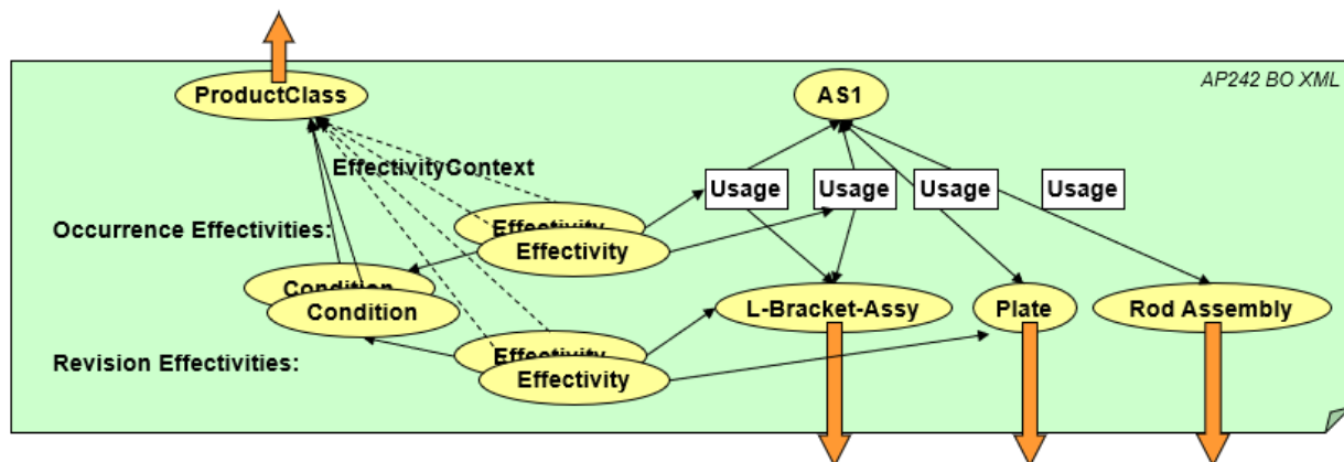
Figure 47: Example for Nested Structure with Effectivities (having a context) making no use of Specifications
