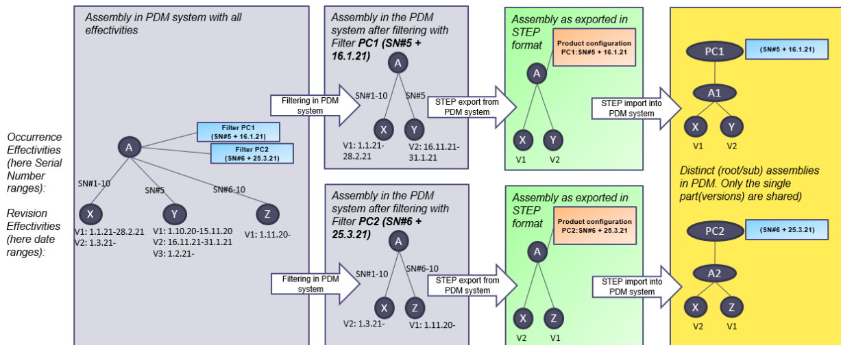
Figure 40: Example for overall process overview for Export of effectivity based single product configuration as explicit assembly structure without effectivities
