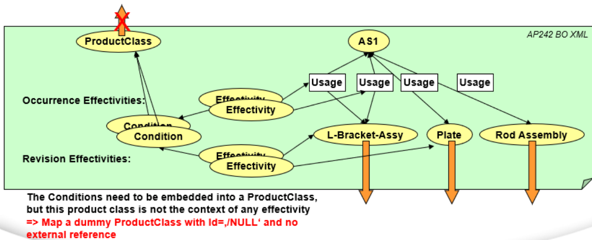
Figure 46: Example for Nested Structure with Effectivities (having no context) with Conditions but making no use of Specifications
