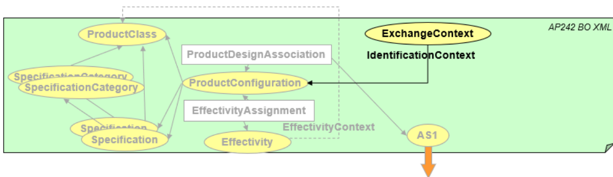
Figure 50: Example for Nested Structure of the product structure filtered for one ProductConfiguration
