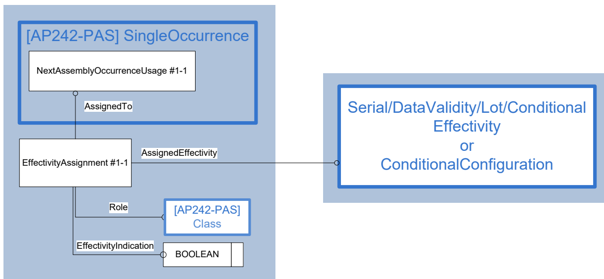
Figure 33: Instance Model EffectivityAssignment for assembly links
