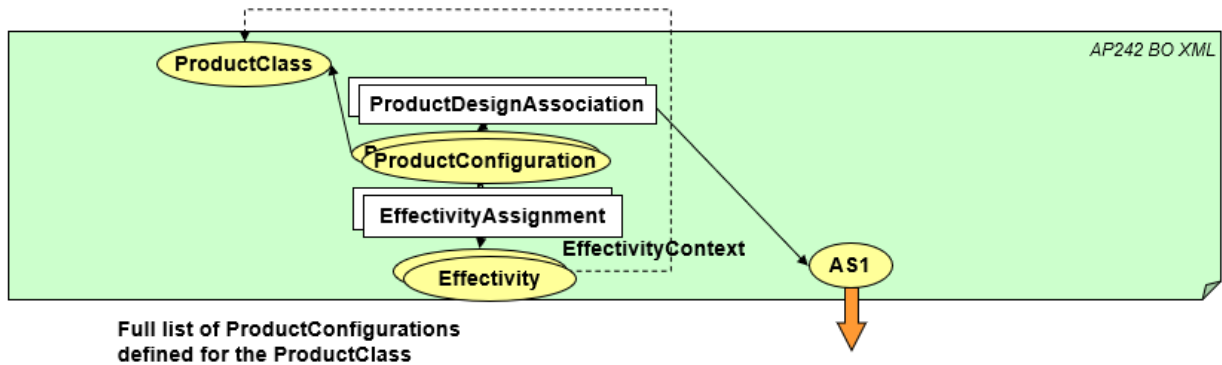
Figure 42: Example for Nested Structure with ProductConfigurations making no use of Specifications
