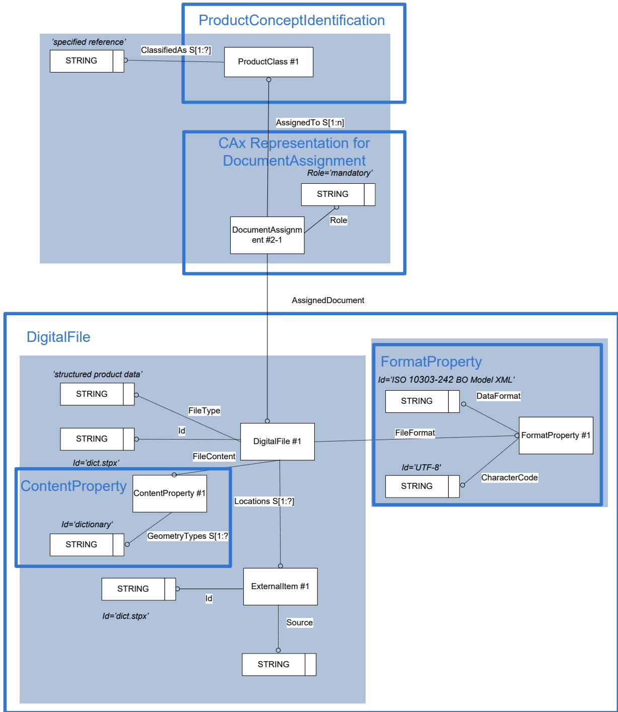
Figure 52: External reference to a ProductClass within a nested XML File containing EffectivityAssignments
