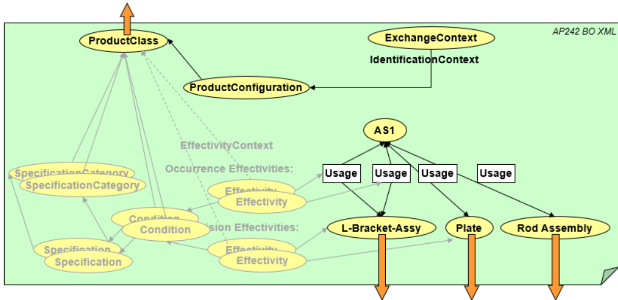
Figure 51: Example for Nested Structure of the product structure filtered of one ProductConfiguration
