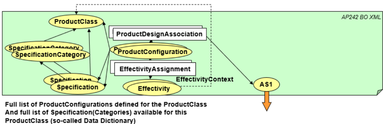
Figure 44: Example for Nested Structure with ProductConfigurations making use of Effectivities and Specifications
