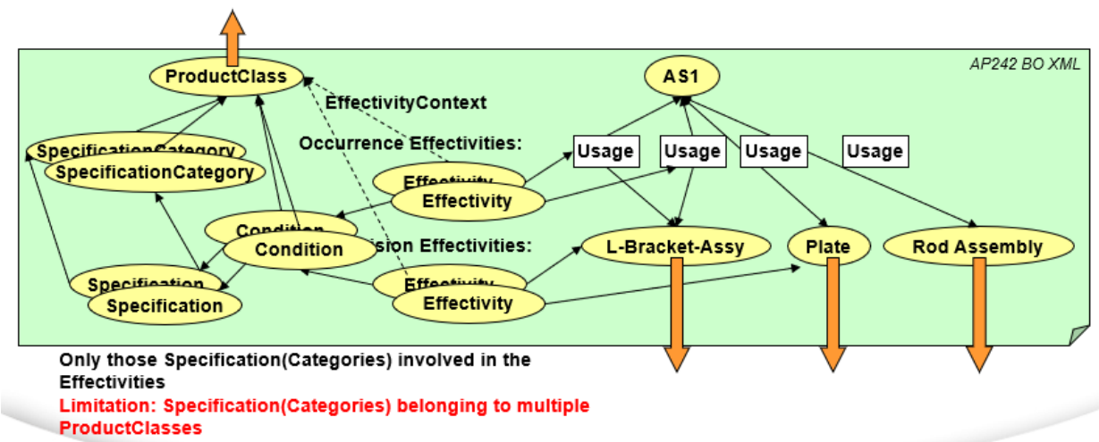
Figure 49: Example for Nested Structure with Effectivities making use of Effectivities and Specifications
