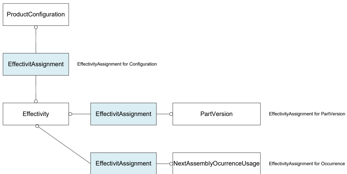
Figure 31: Simplified Example for supported EffectivityAssignments
