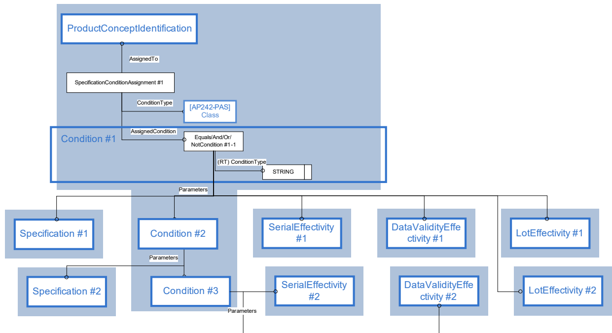
Figure 39: Instance Model SpecificationConditionAssignment
