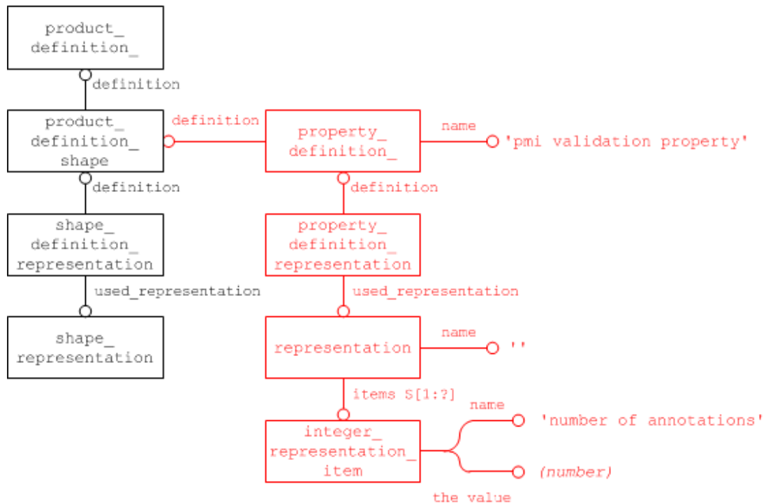
Figure 113: PMI Validation Property for total number of annotations per part
