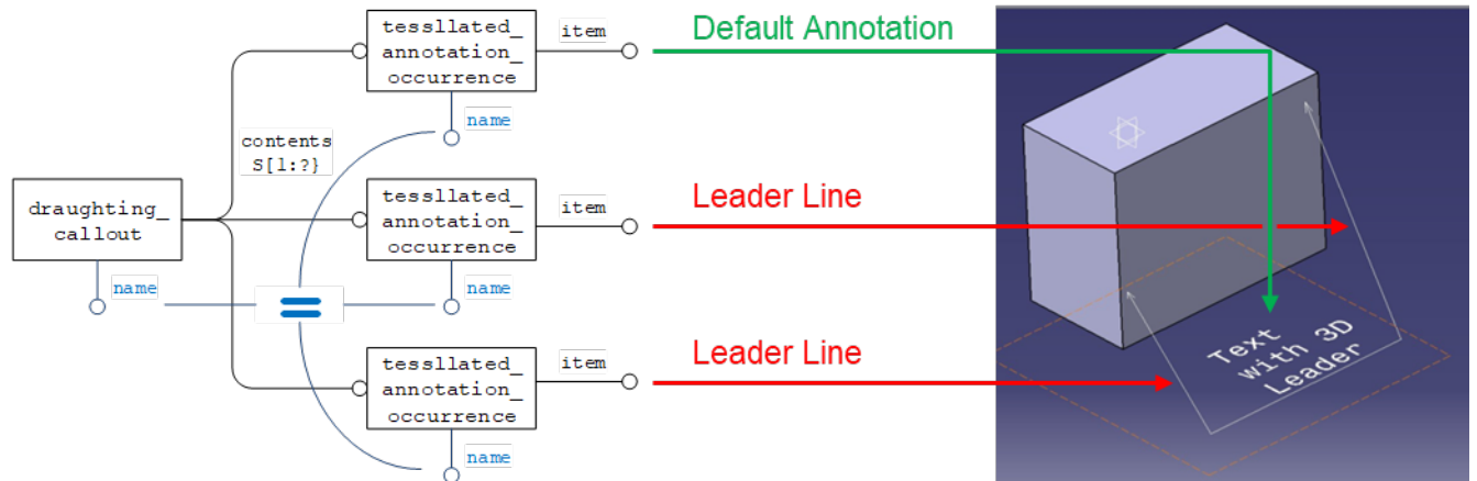
Figure 83: Graphic Annotation Subsets for non-coplanar Annotations
