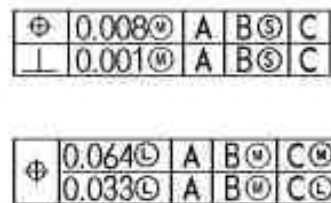
Figure 107: Stacked Tolerances (top) vs. Composite Tolerance (bottom)
