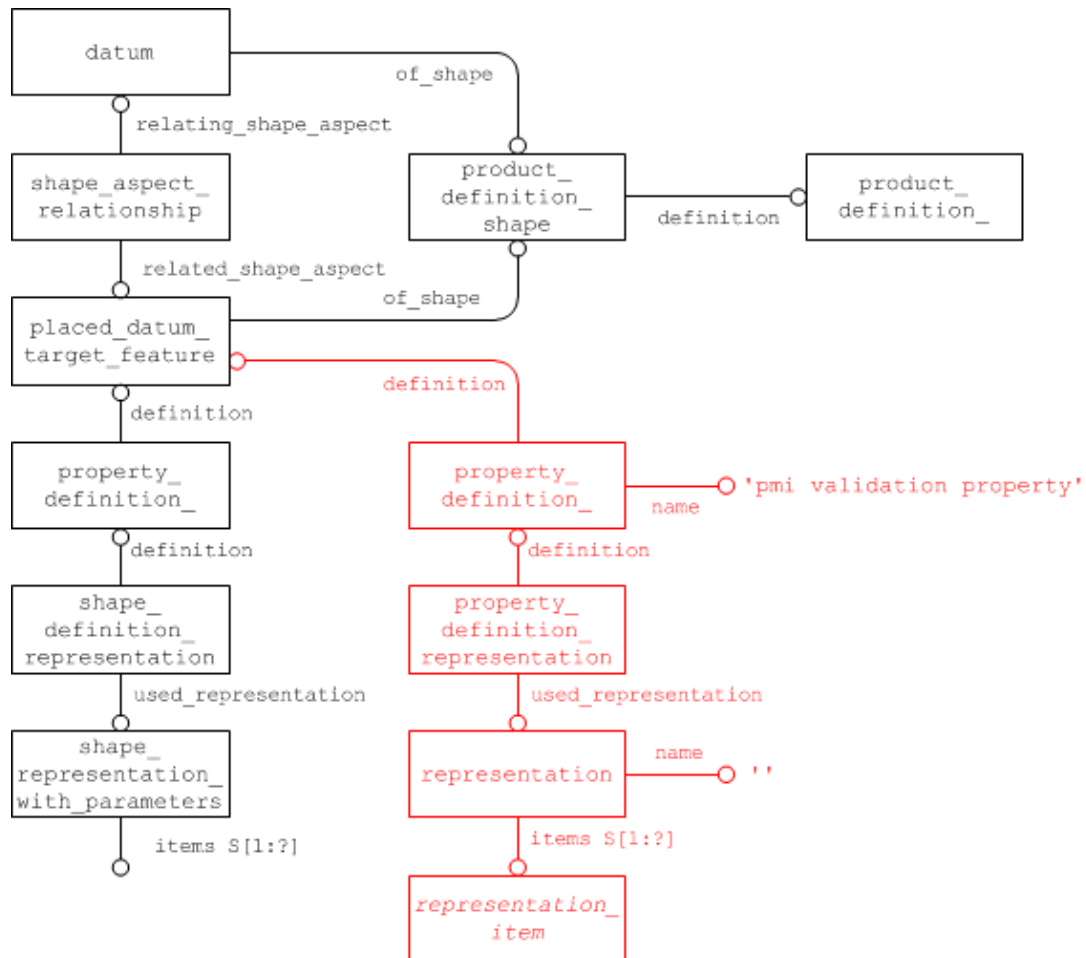
Figure 112: Validation Property for Placed Datum Target Feature
