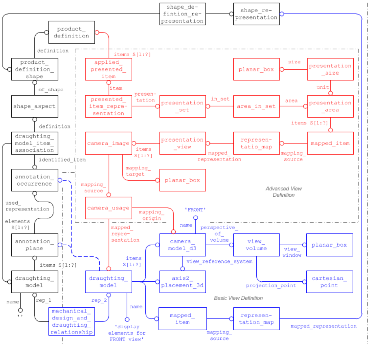
Figure 105: Advanced Saved View Implementation
