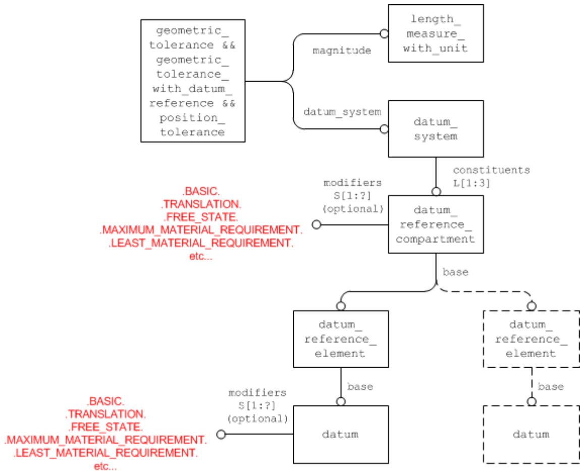
Figure 68: Common/Multiple Datum Instantiation
