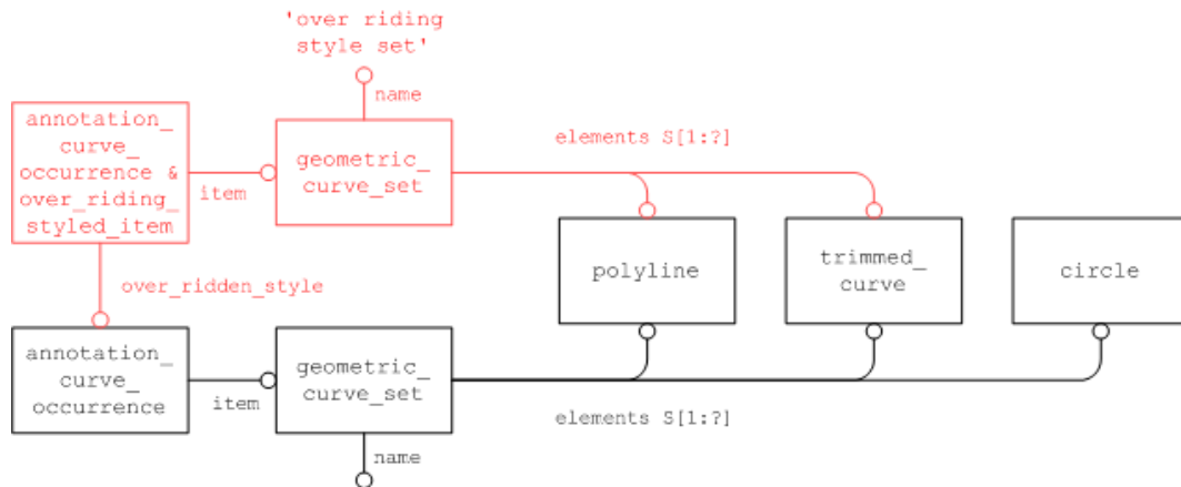
Figure 85: Definition of the overriding style for a Polyline annotation
