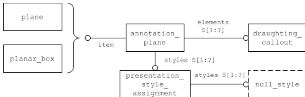
Figure 86: Definition of the view plane
