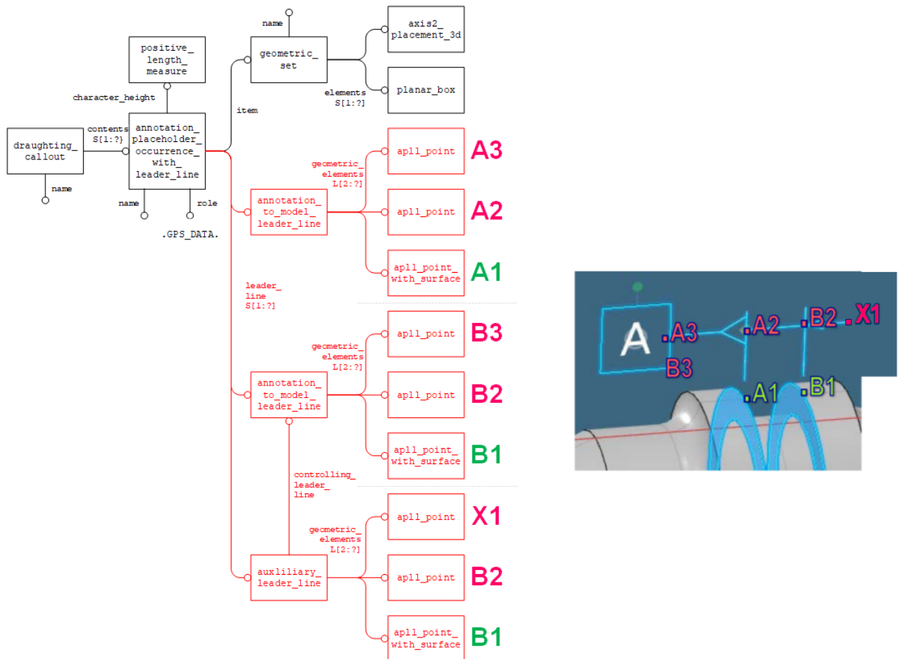
Figure 74: Presentation Placeholder with Leader Lines Example
