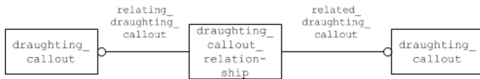
Figure 91: Linking Annotations to other Annotations
