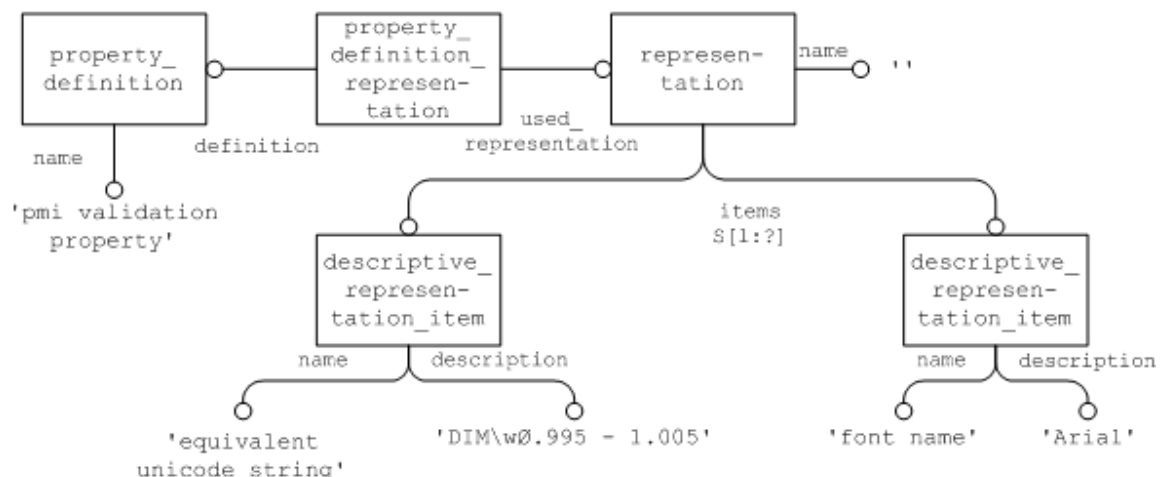
Figure 119: Equivalent Unicode String validation property
