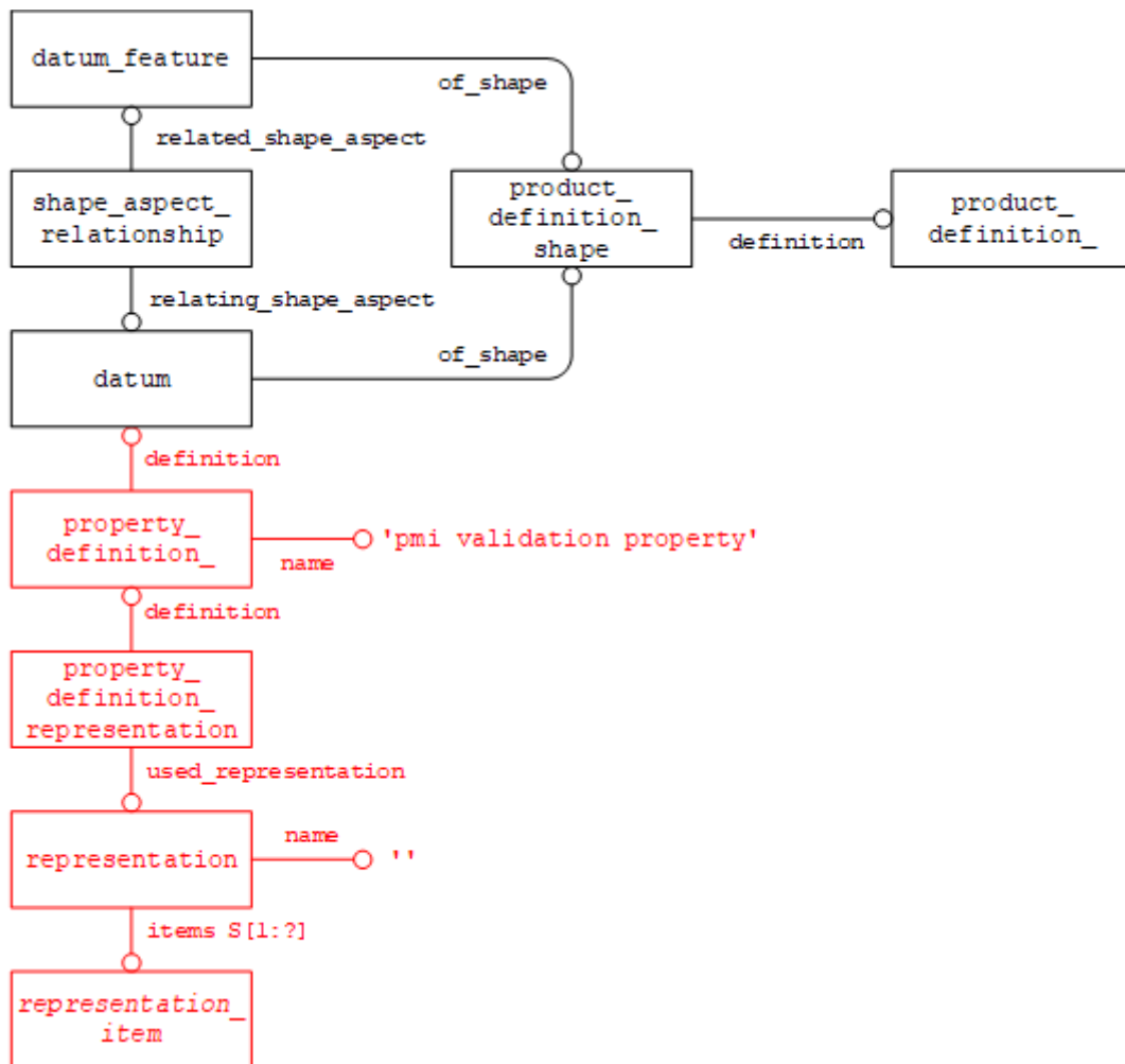
Figure 111: Validation Property for Datum Feature
