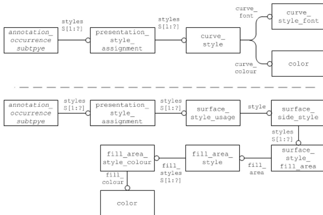
Figure 84: Styling a Graphic Annotation for outline/stroked (top) and filled (bottom) Elements
