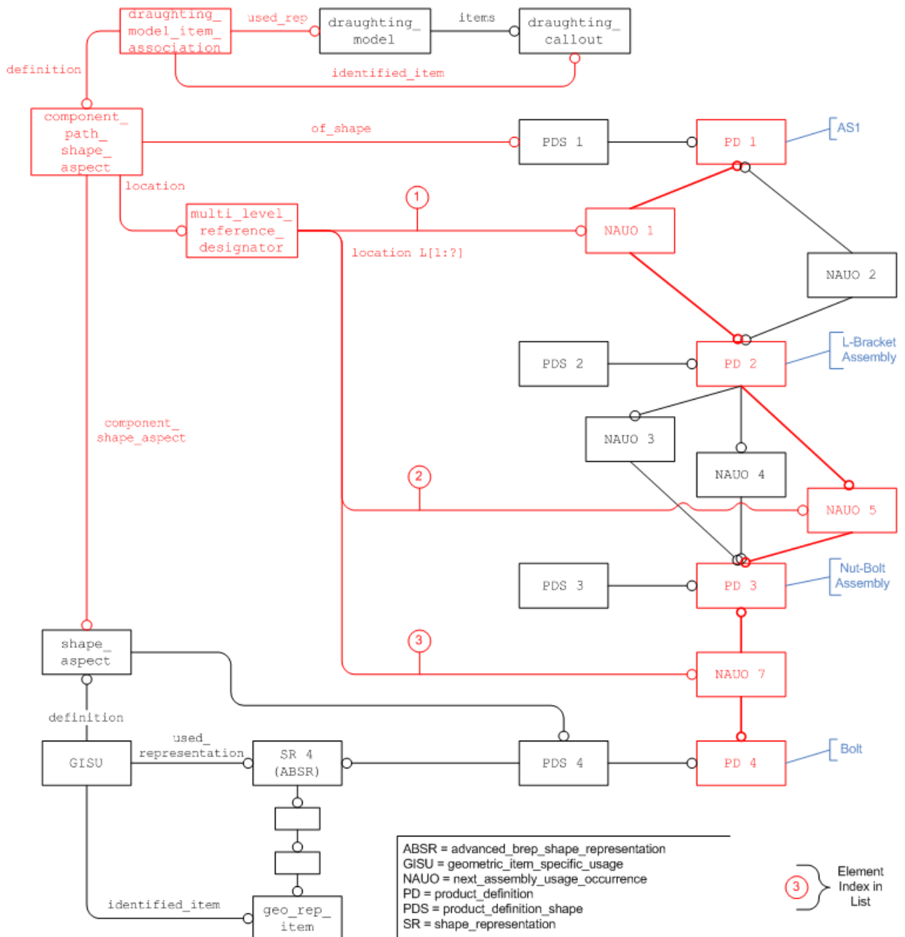
Figure 94: Linking annotation to a component instance in an assembly
