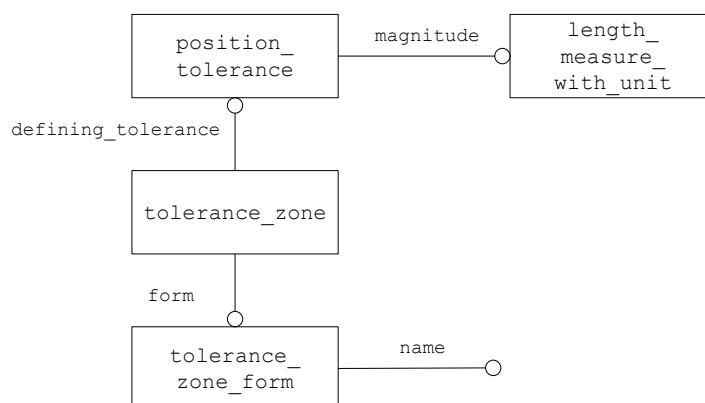
Figure 49: Tolerance Zone
