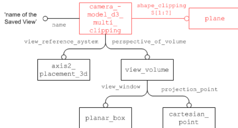
Figure 101: Definition of a Section View using a single Plane
