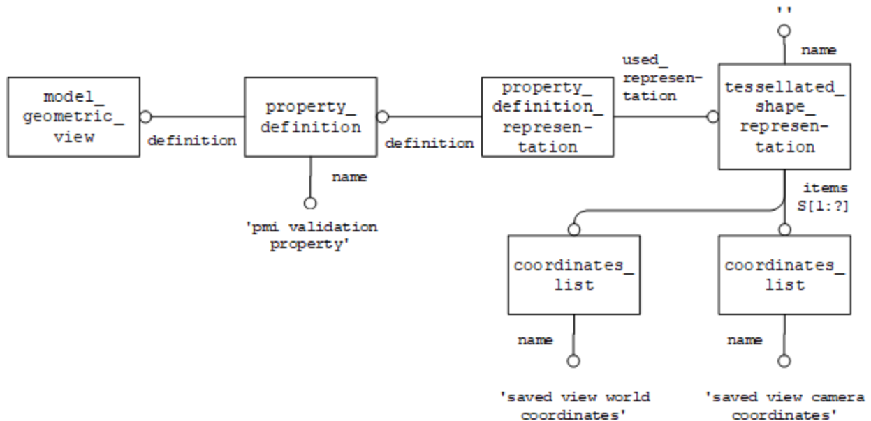
Figure 116: PMI Validation Property for Camera Position
