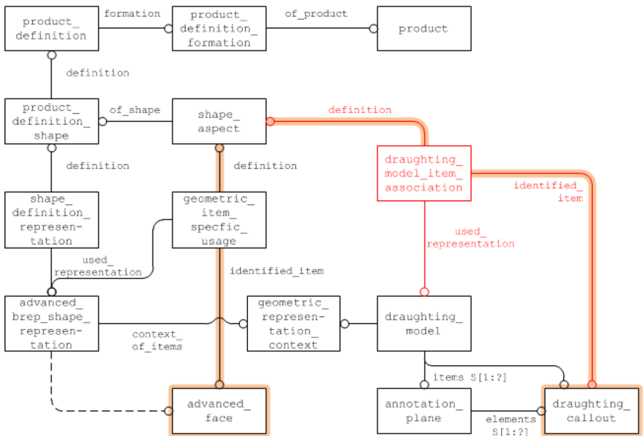
Figure 89: Associating the Annotation with the Geometry
