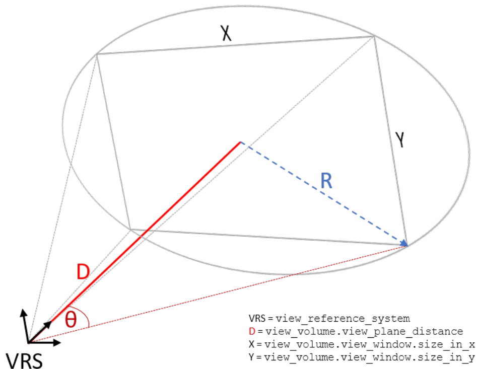
Figure 117: Determining the Zoom Factor for a Saved View
