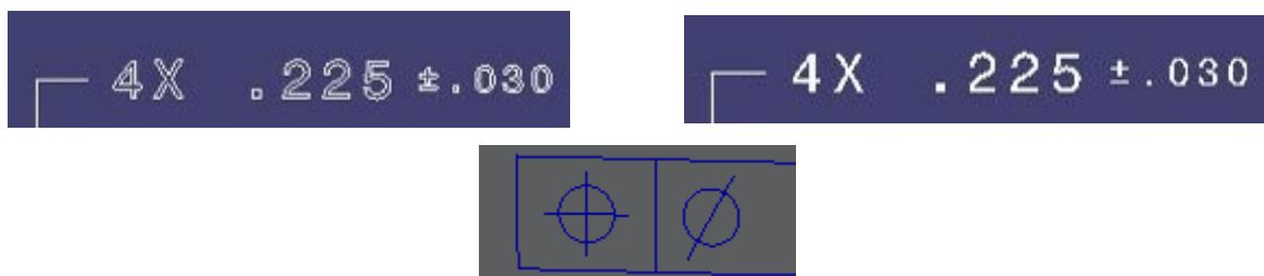
Figure 77: Outline Characters (upper left), Filled Characters (upper right), Stroked Characters and Geometric Elements (below)
