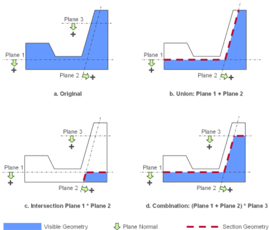
Figure 102: Schematic representation of possible clipping cases
