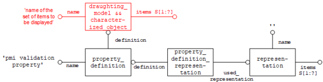
Figure 114: Defining PMI Validation Properties for the contents of a Saved View
