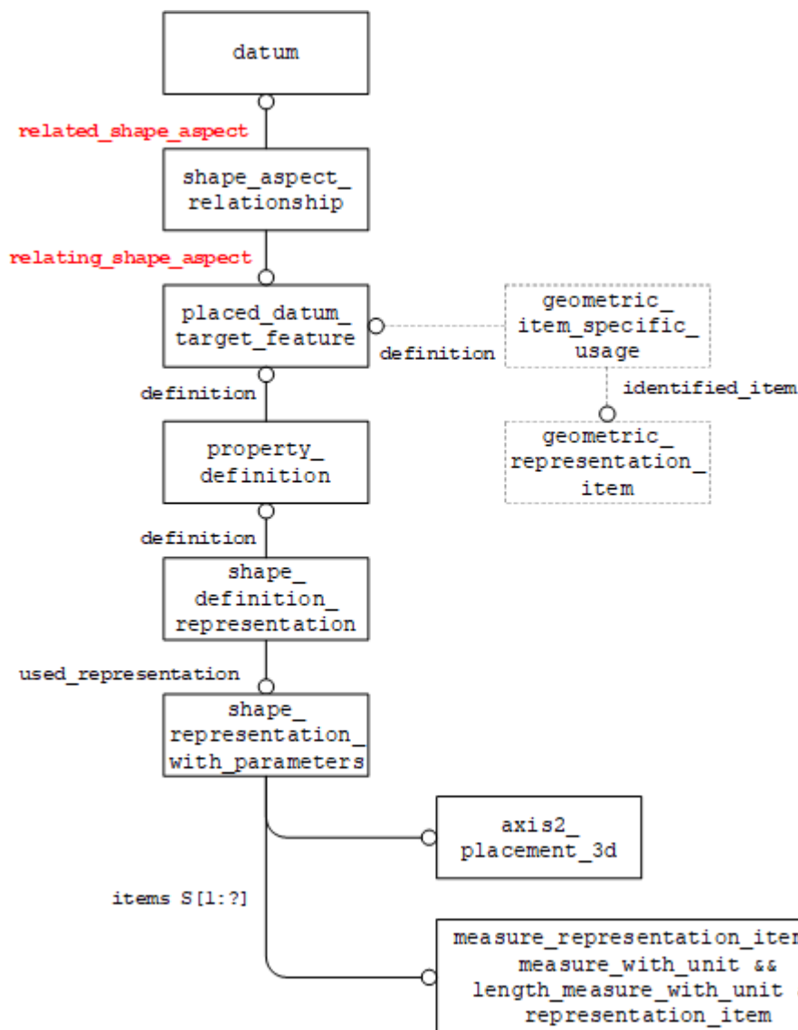
Figure 43: Datum Target Instantiation
