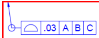
Figure 32: Example Tolerance with All Around Modifier
