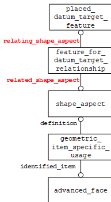
Figure 45: Relating Datum Target to Feature
