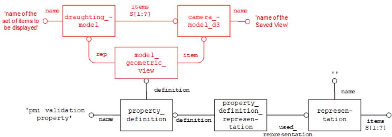
Figure 115: Defining PMI Validation Properties for the perspective of a Saved View
